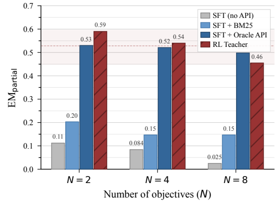
Figure 5: em\_partial under different retrieval conditions. Providing oracle retrieval results at inference time recovers the SFT student from near-zero to near-teacher performance across all N , while even a standard BM25 backend yields meaningful gains. The RL teacher (hatched) is shown for reference.
