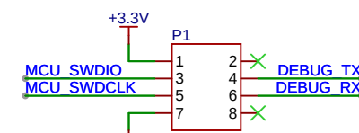
GND SWD烧写调试
