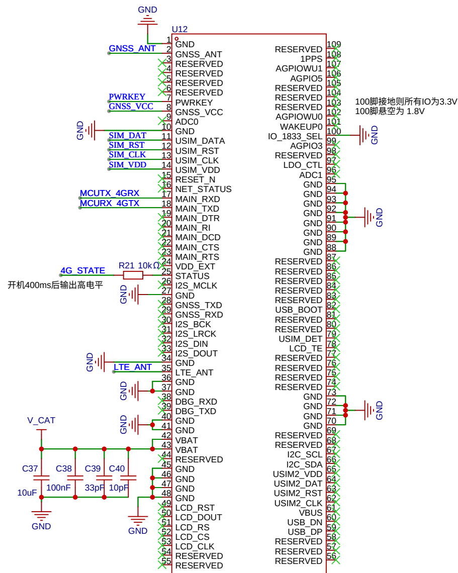
Air780EG 4G-CAT1模块
