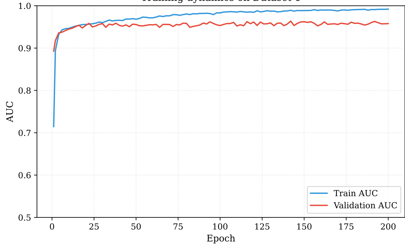
Training dynamics on Dataset 1
