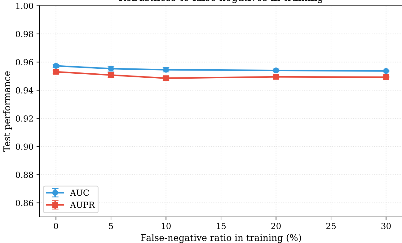
Robustness to false negatives in training
