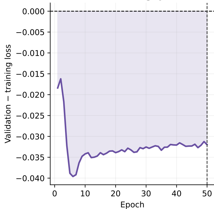
B. Generalization gap
