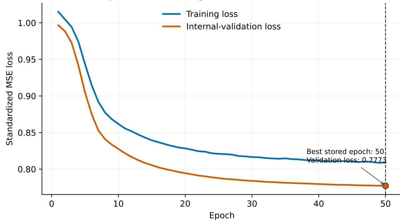
A. Multi-output MLP learning curves
