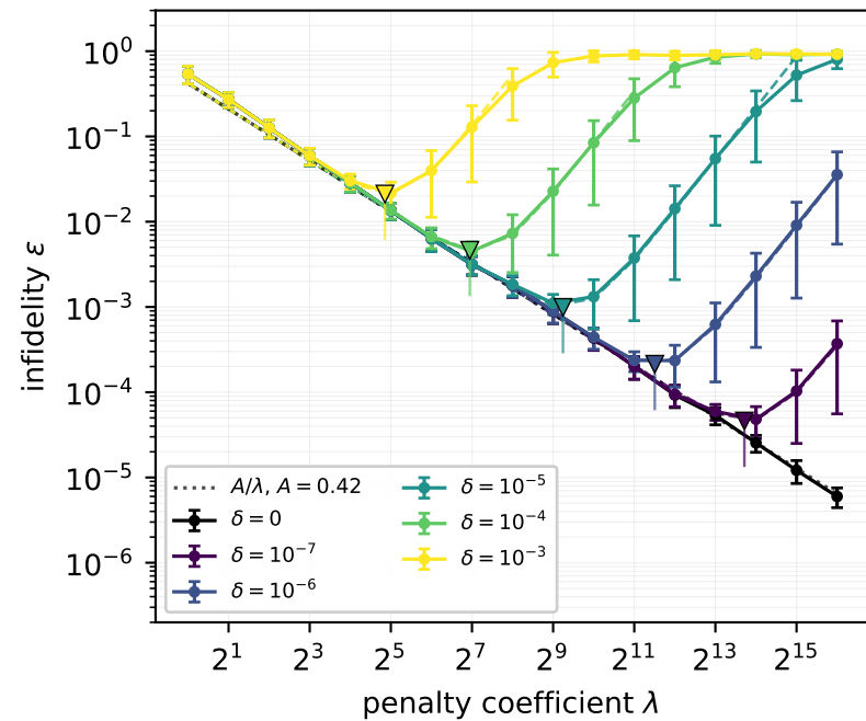
(a) n_b = 2 , t = 1 , 1-local noise 0.1
