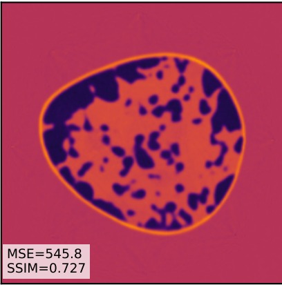
Naive-CBS8
