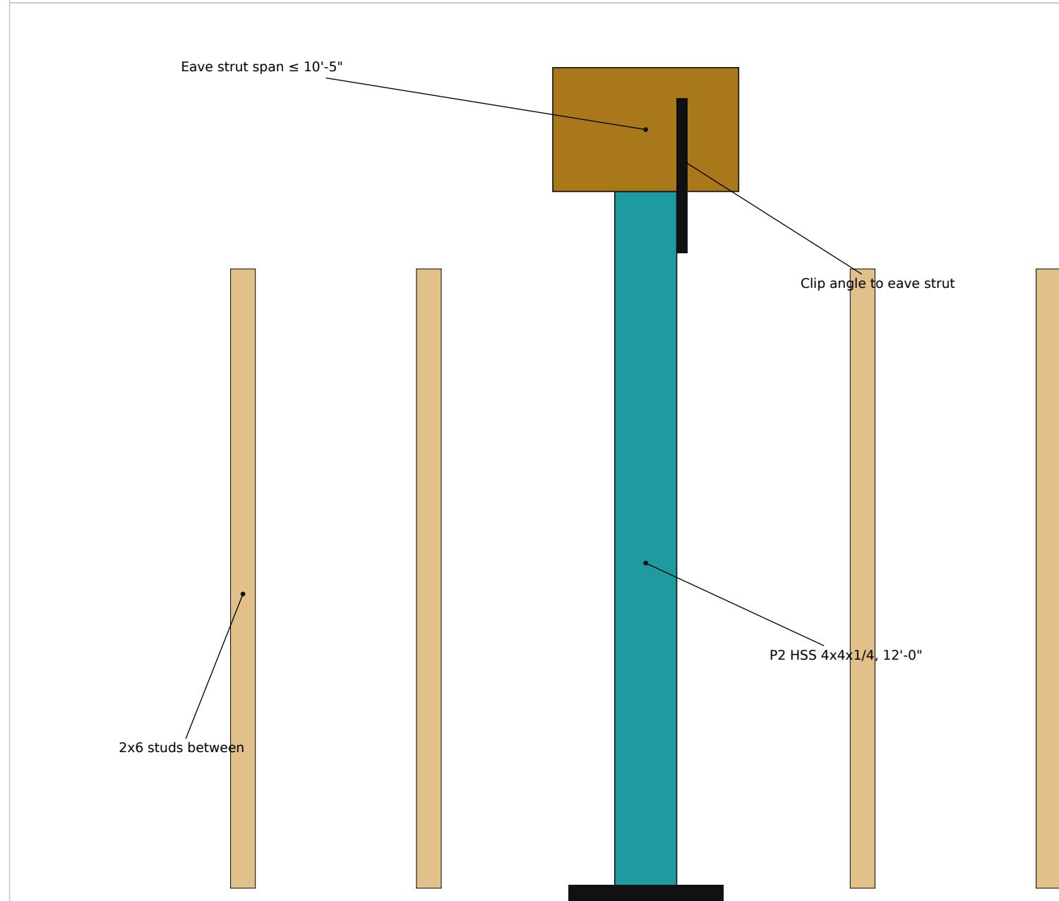
8 MID-BAY WIND POST SCALE: NTS
