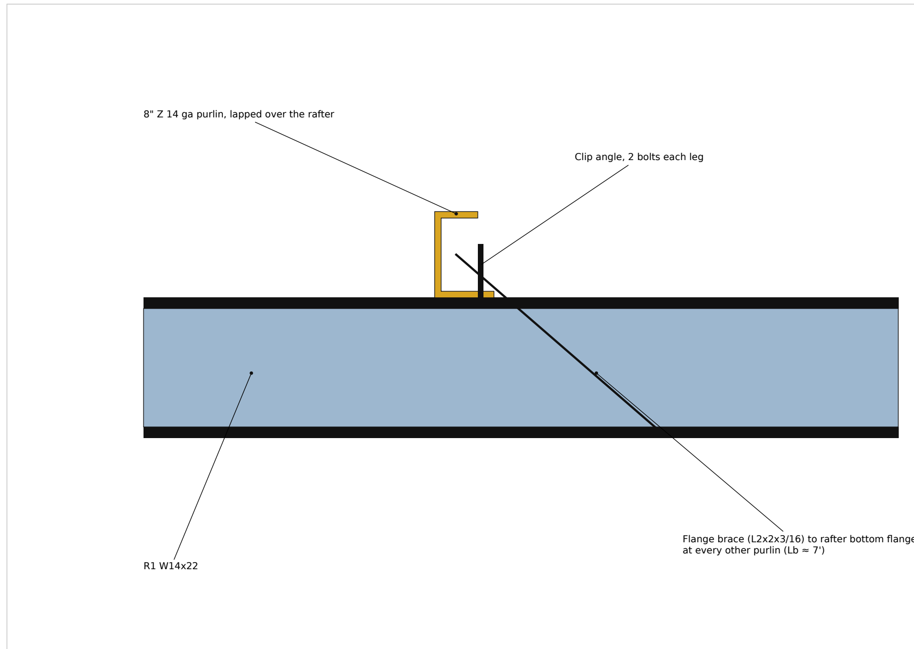
5 PURLIN AND FLANGE BRACE SCALE: NTS
