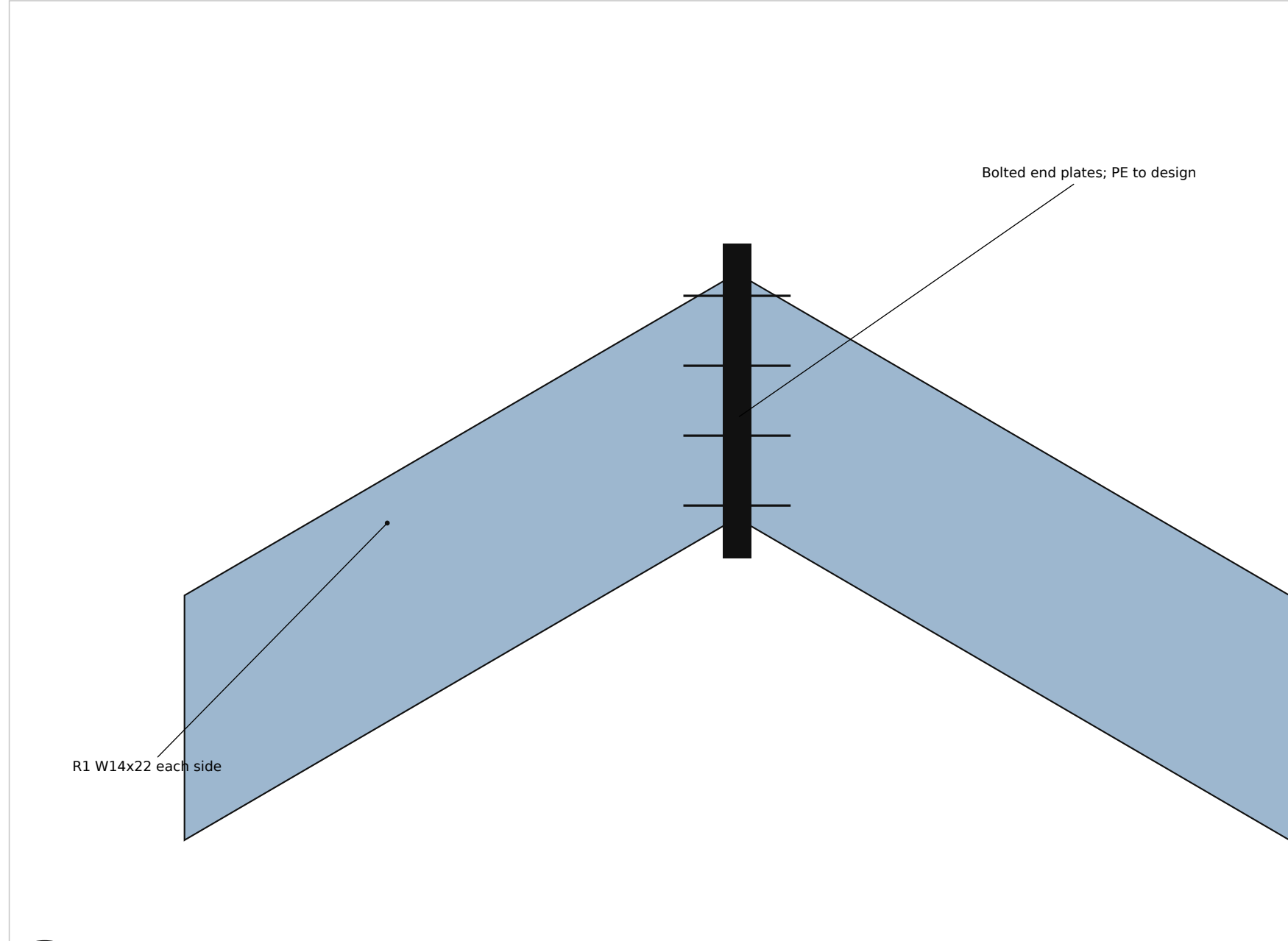
3 RIDGE SPLICE SCALE: NTS
