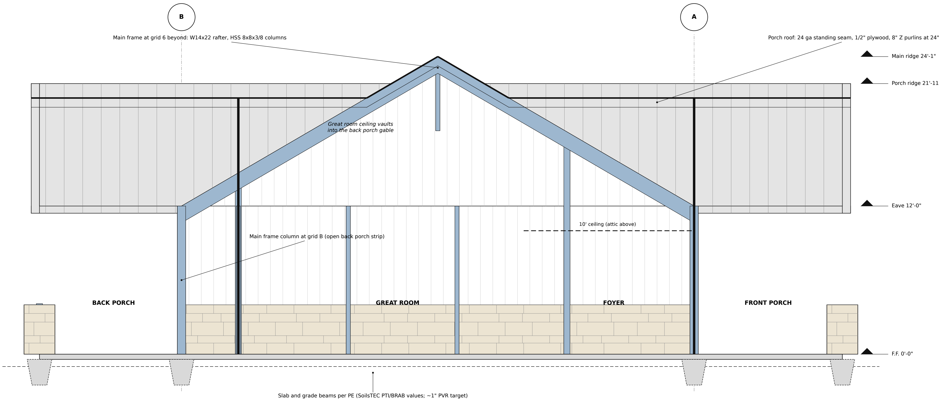
1 SECTION 1 — FOYER AND GREAT ROOM SCALE: 1/4" = 1'-0"
