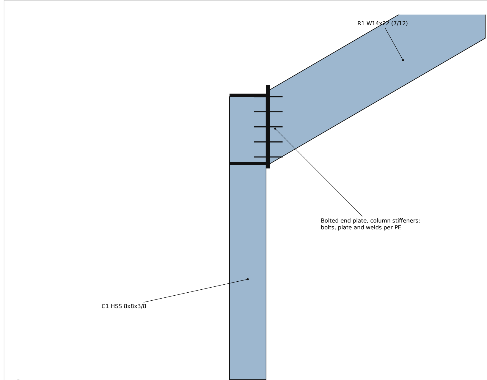
2 KNEE MOMENT CONNECTION SCALE: NTS
