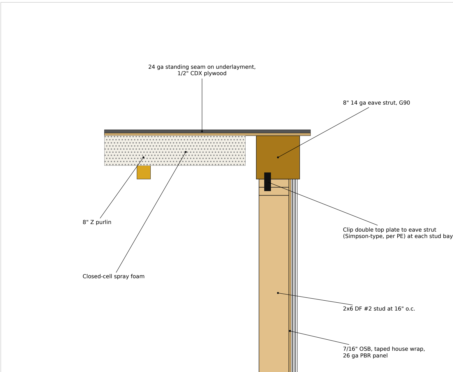
4 EAVE: WOOD WALL TO STEEL SCALE: NTS
