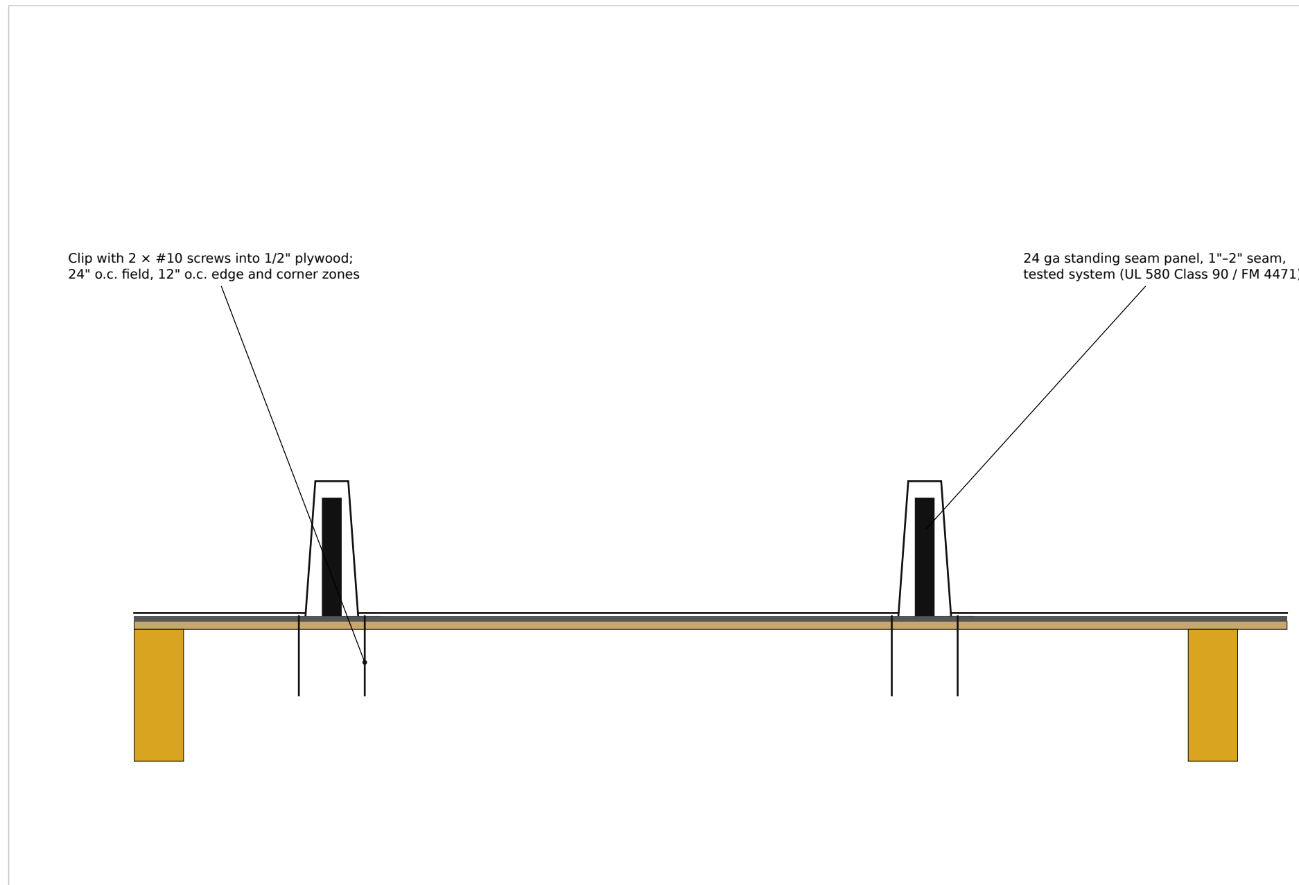
6 STANDING SEAM CLIP SCALE: NTS
