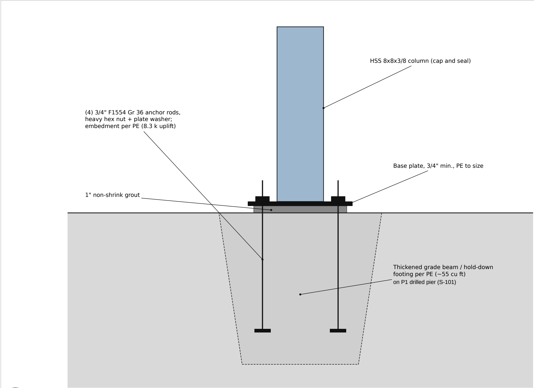
1 COLUMN BASE PLATE (BP-1) SCALE: NTS
