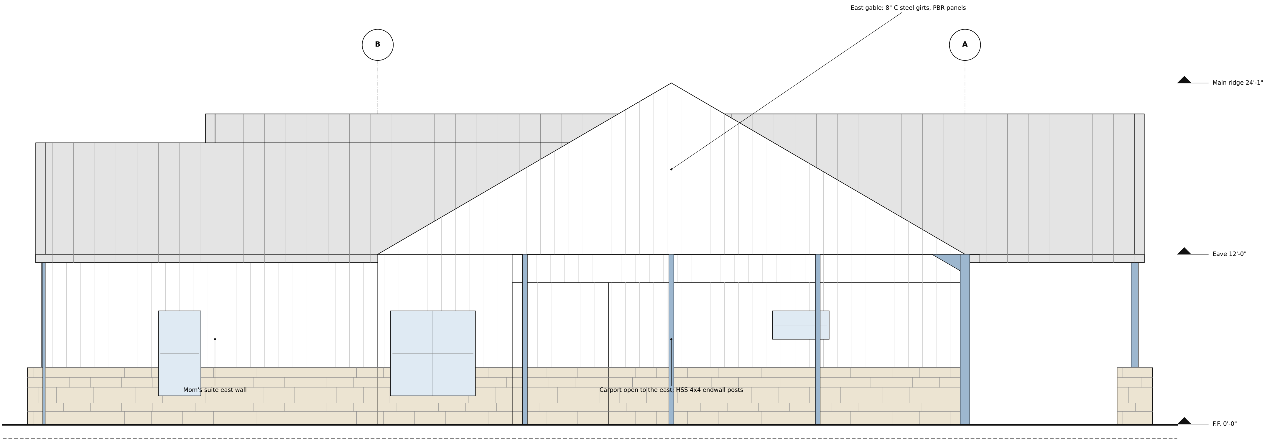
1 EAST ELEVATION (CARPORT SIDE) SCALE: 1/4" = 1'-0"
