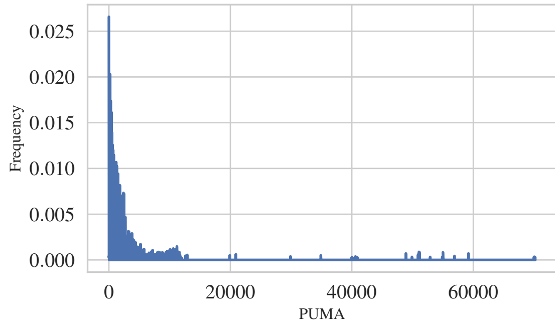
K=70201, N=1664500
