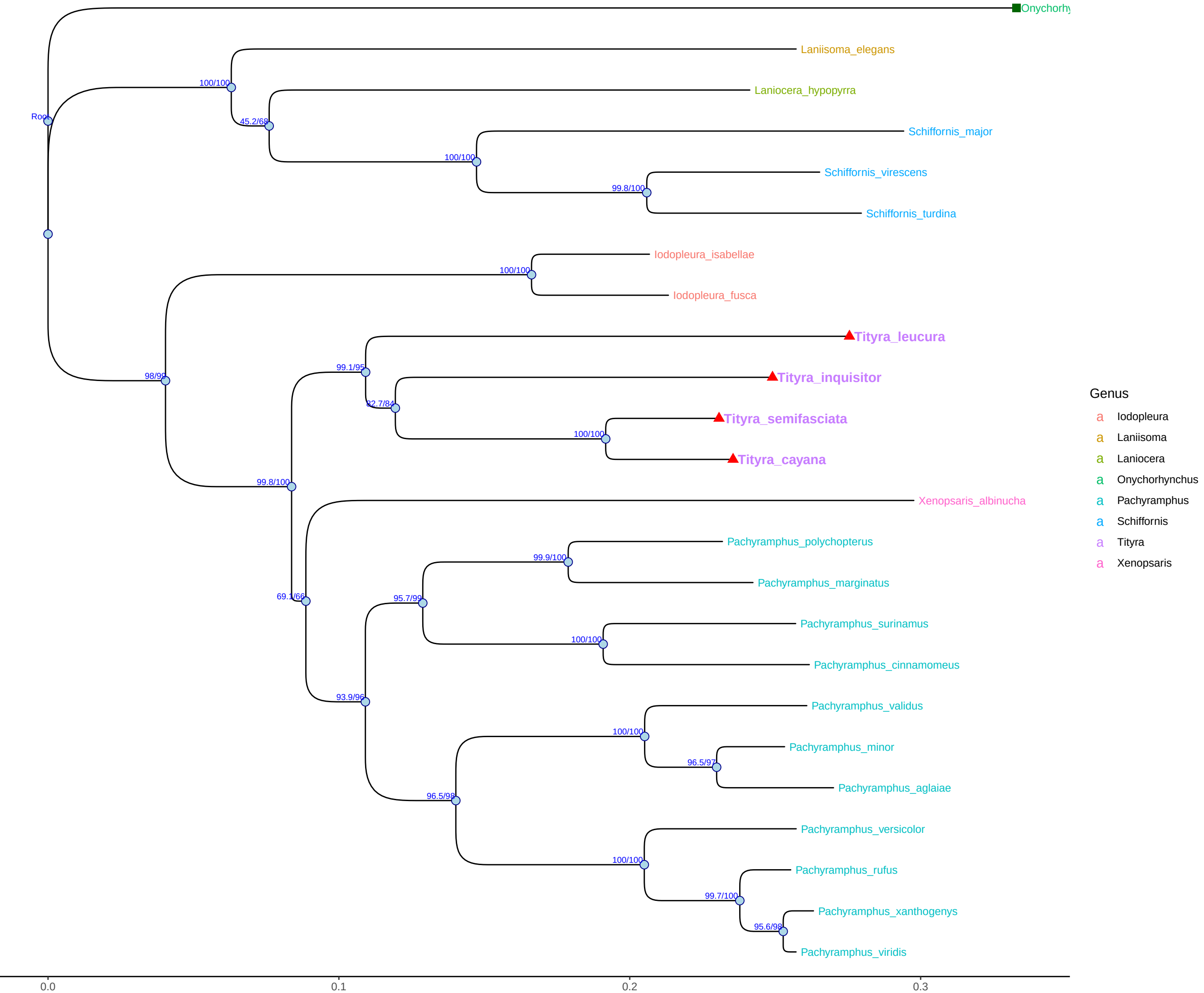
Concatenated Genes Phylogeny with Bootstrap Support (Rooted with Onychorhynchus)
