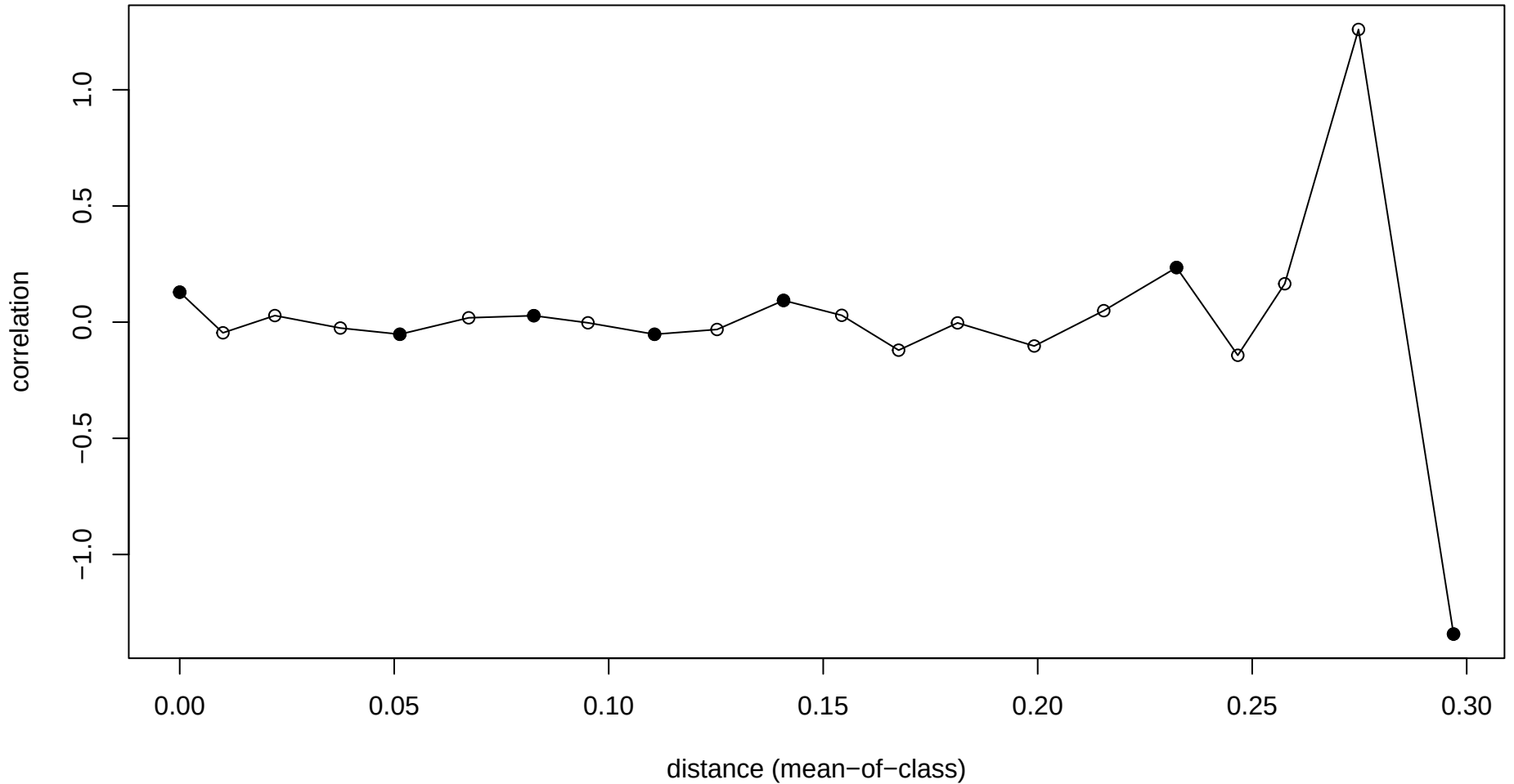
Moran's I Correlogram – Shannon Diversity
