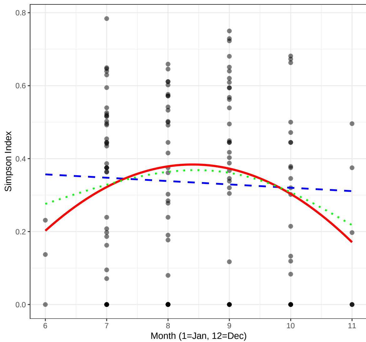
Evenness: Model Comparison (Repeated Sites)
