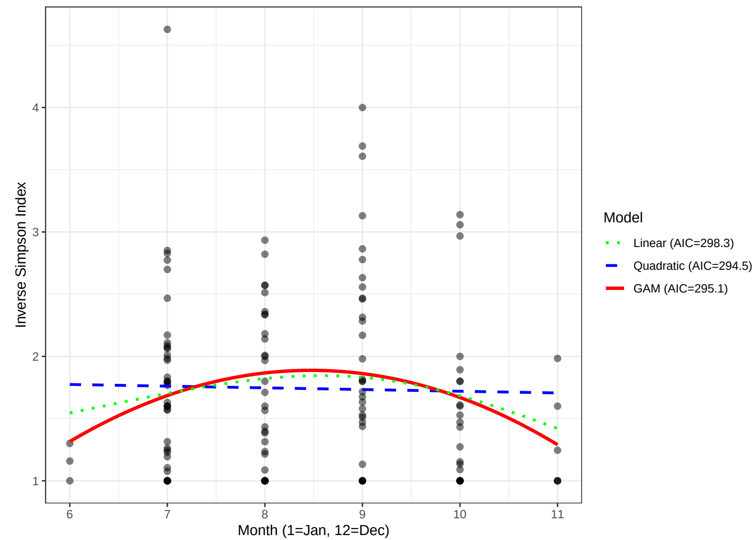
Inverse Simpson: Model Comparison (Repeated Sites)
