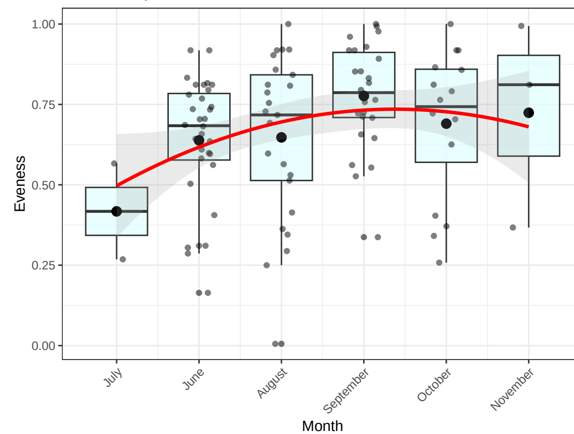
Evenness by Month – Repeated Sites (with Quadratic Fit)
