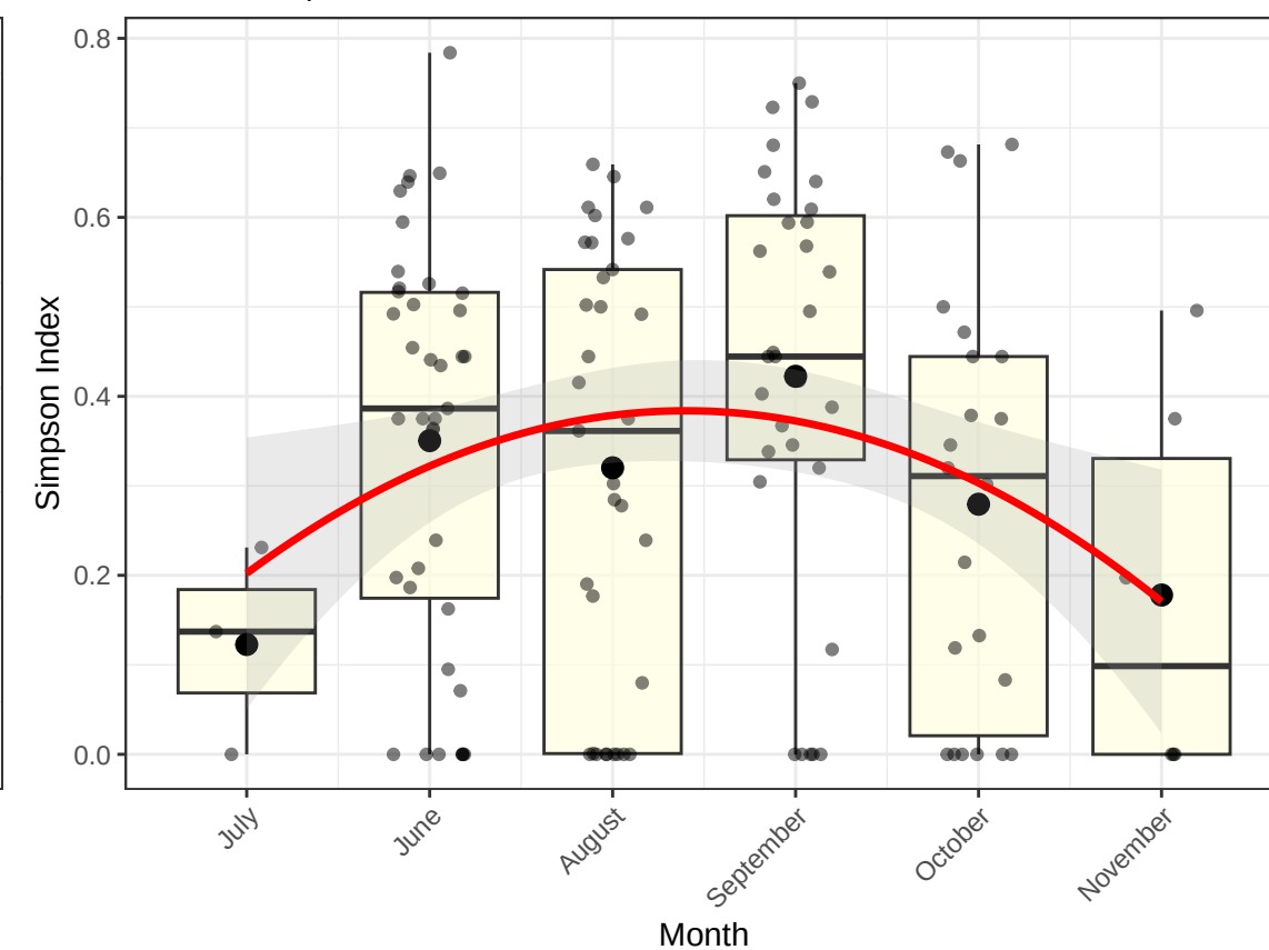
Simpson Diversity by Month – Repeated Sites (with Quadratic Fit)
