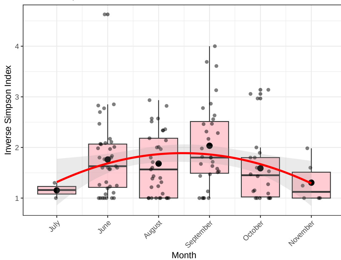
Inverse Simpson Diversity by Month – Repeated Sites (with Quadratic Fit)
