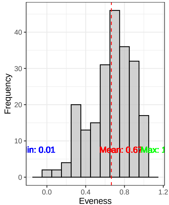
Histogram of Evenness
