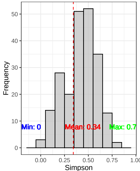
Histogram of Simpson
