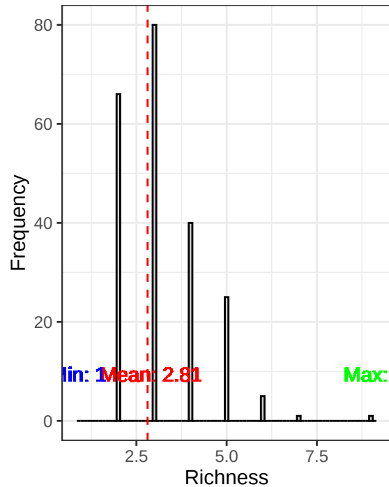
Histogram of Richness
