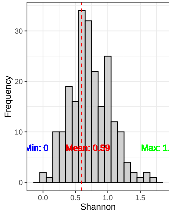
Histogram of Shannon
