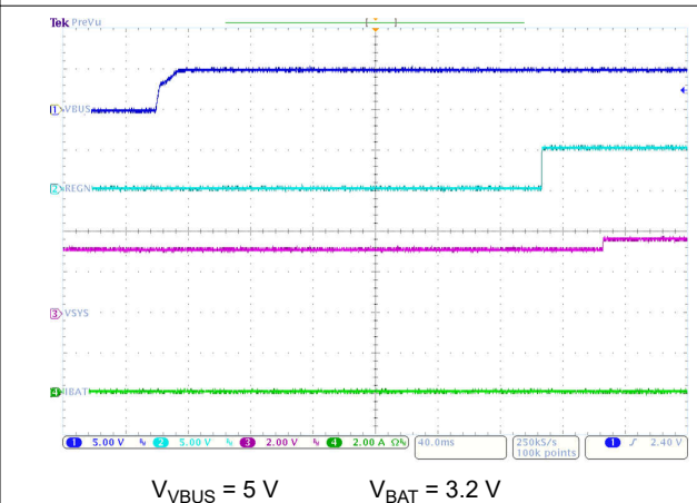
Figure 8-5. Power Up with Charge Disabled
