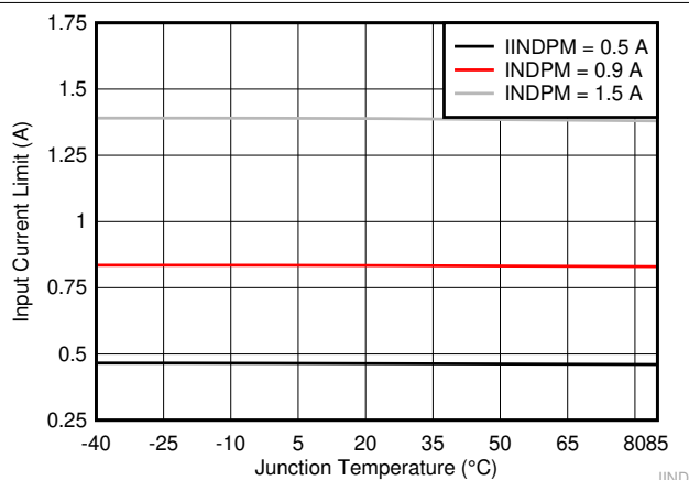
Figure 6-10. Input Current Limit vs Junction Temperature
