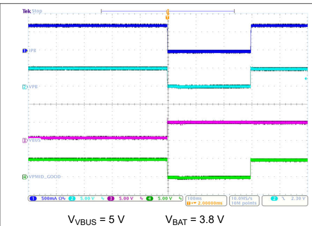
Figure 8-3. VBUS Plugged In with Boost Mode Enabled
