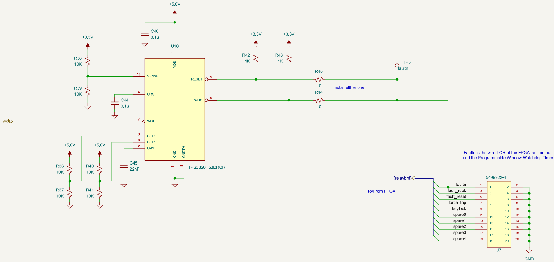
Programmable Window Watchdog Timer
