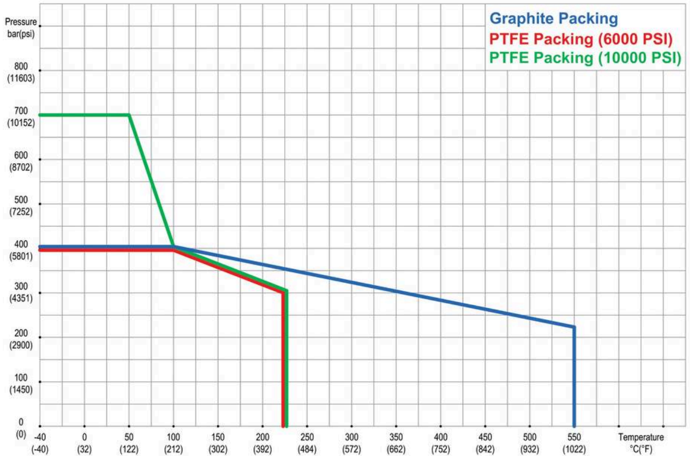
P-T CHART FOR NEEDLE VALVE & MANIFOLD VALVE
