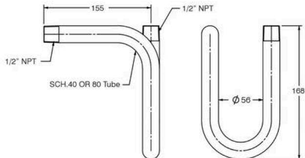
"U" Type Siphon
