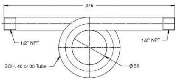
Pigtail Type Siphon
