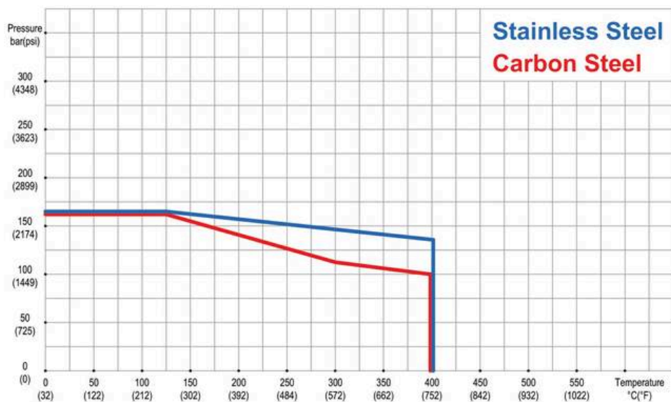
P-T CHART FOR SYPHON (COIL TYPE & U TYPE)
