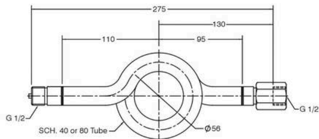
Coil Type Siphon
