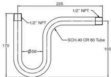
Flat "U" Type Siphon
