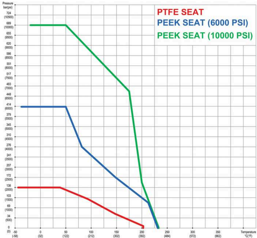
P-T CHART FOR BALL VALVE SEAT
