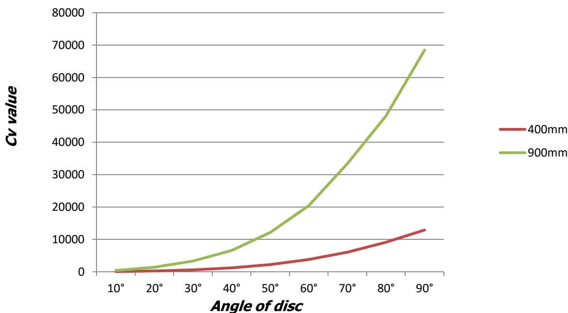
Flow through BAF Butterfly Valve, size 400mm and 900mm
