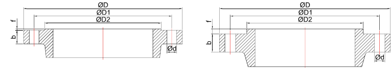
Class 150 to 300LB
