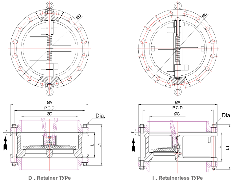
Dual Plate Flange Type Check Valve
