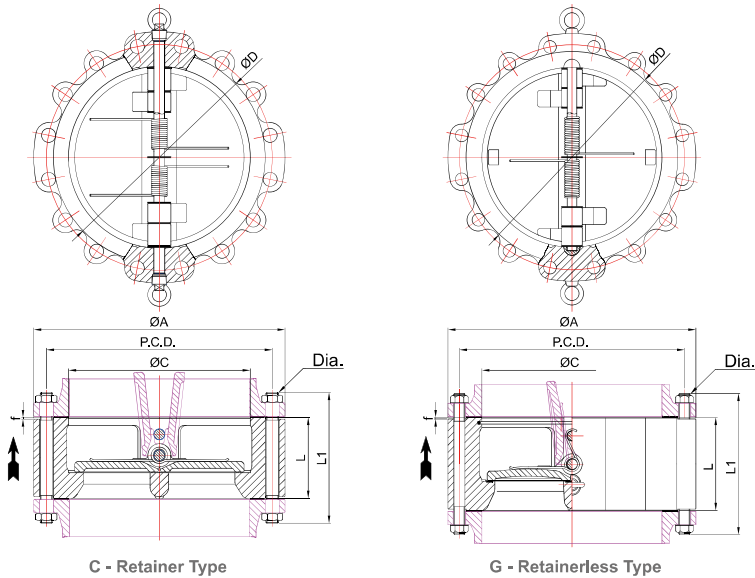
Dual Plate Lug Type Check Valve
