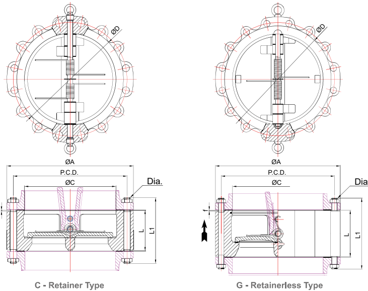
Dual Plate Lug Type Check Valve
