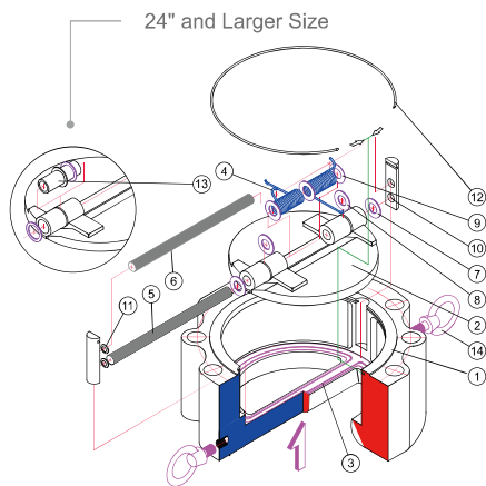
Retainerless Type ( G Type )
