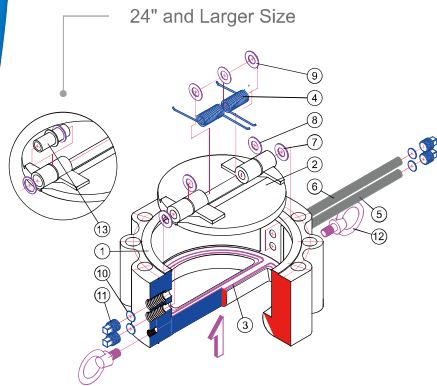
Retainer Type ( C Type )
