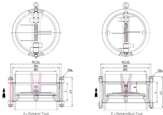
Dual Plate Wafer Type Check Valve
