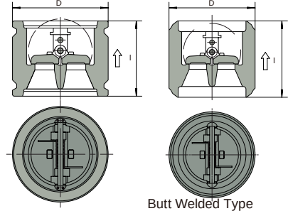
Hub Ended Type
