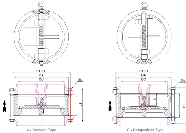
Dual Plate Wafer Type Check Valve
