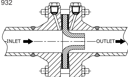
Flow Nozzle Mounted Between Flanges
