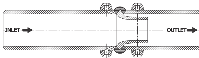
ISA 1932, WELDIN TYPE
