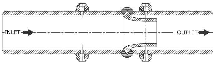
Long Radius High Beta, Weldin Type
