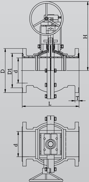
SECTIONAL VIEW
