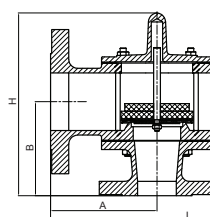
PR2 Weight-Loaded
