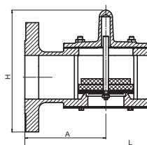
VR2 Weight-Loaded
