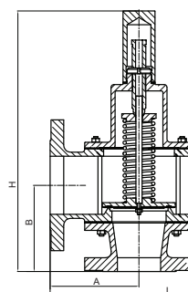
PR2S Spring-Loaded
