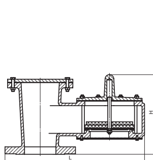
VR1 Weight-Loaded
