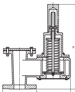
VR1S Spring-Loaded
