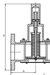
VR2S Spring-Loaded
