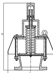
PR1S Spring-Loaded
