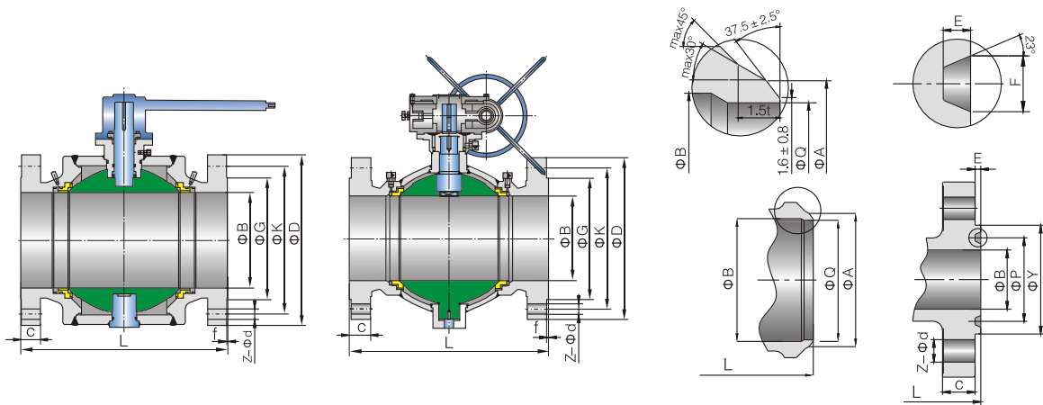
Main Connection Dimension
