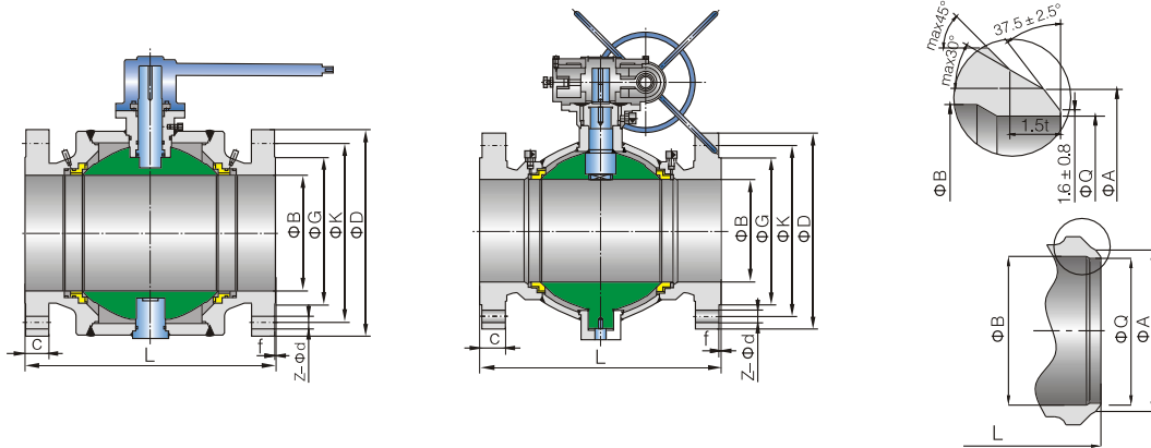
Main Connection Dimension
