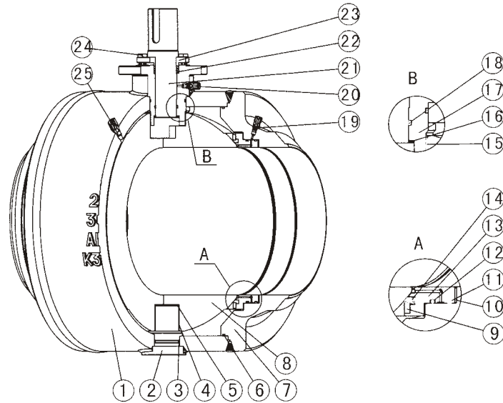
Valve Structural Schematic Drawing (Forge Welded Structure)
