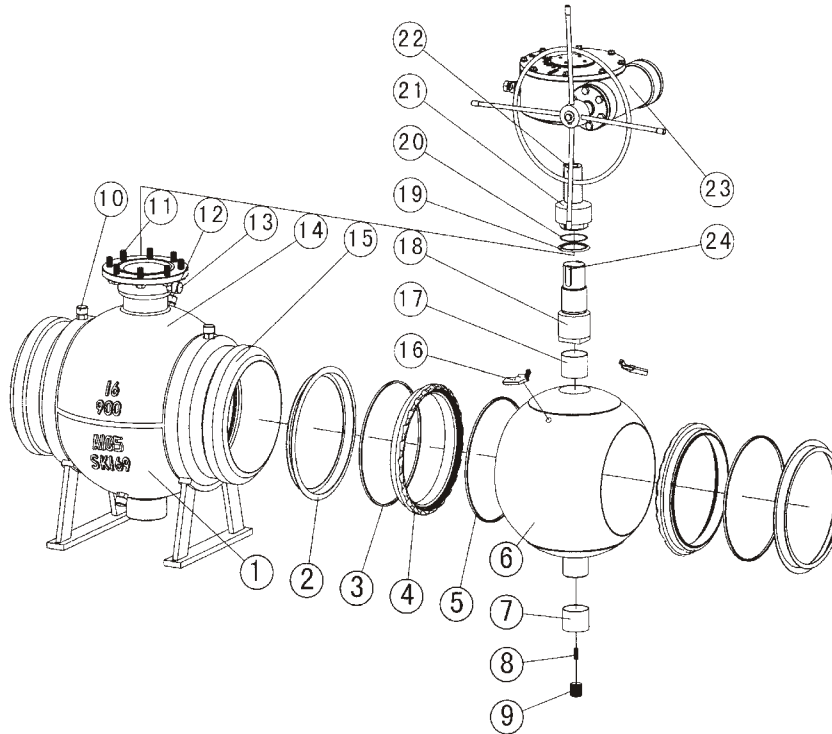
The Material of Main Parts (Plate Welded and Cast Welded)
