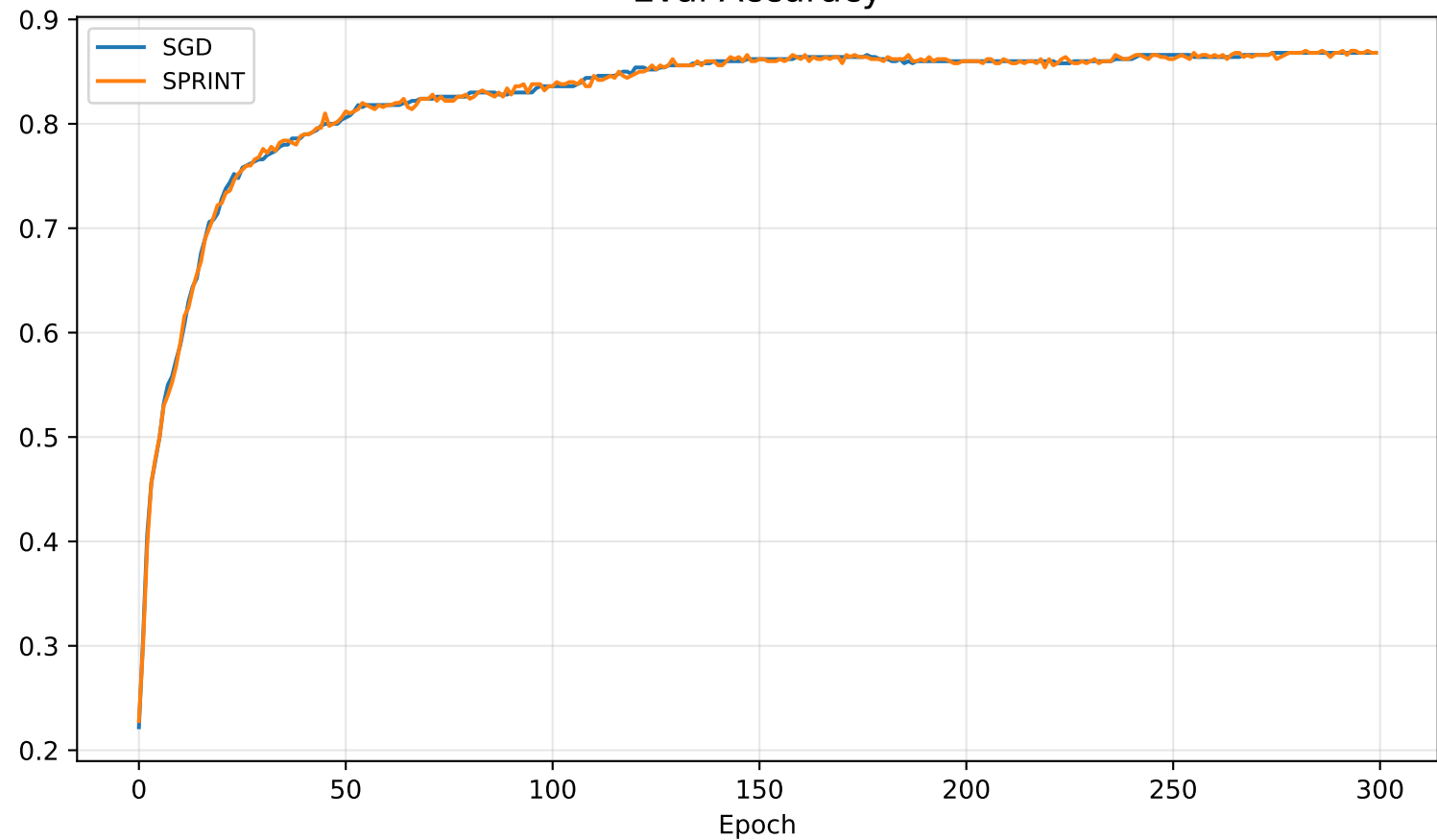
Eval Accuracy
