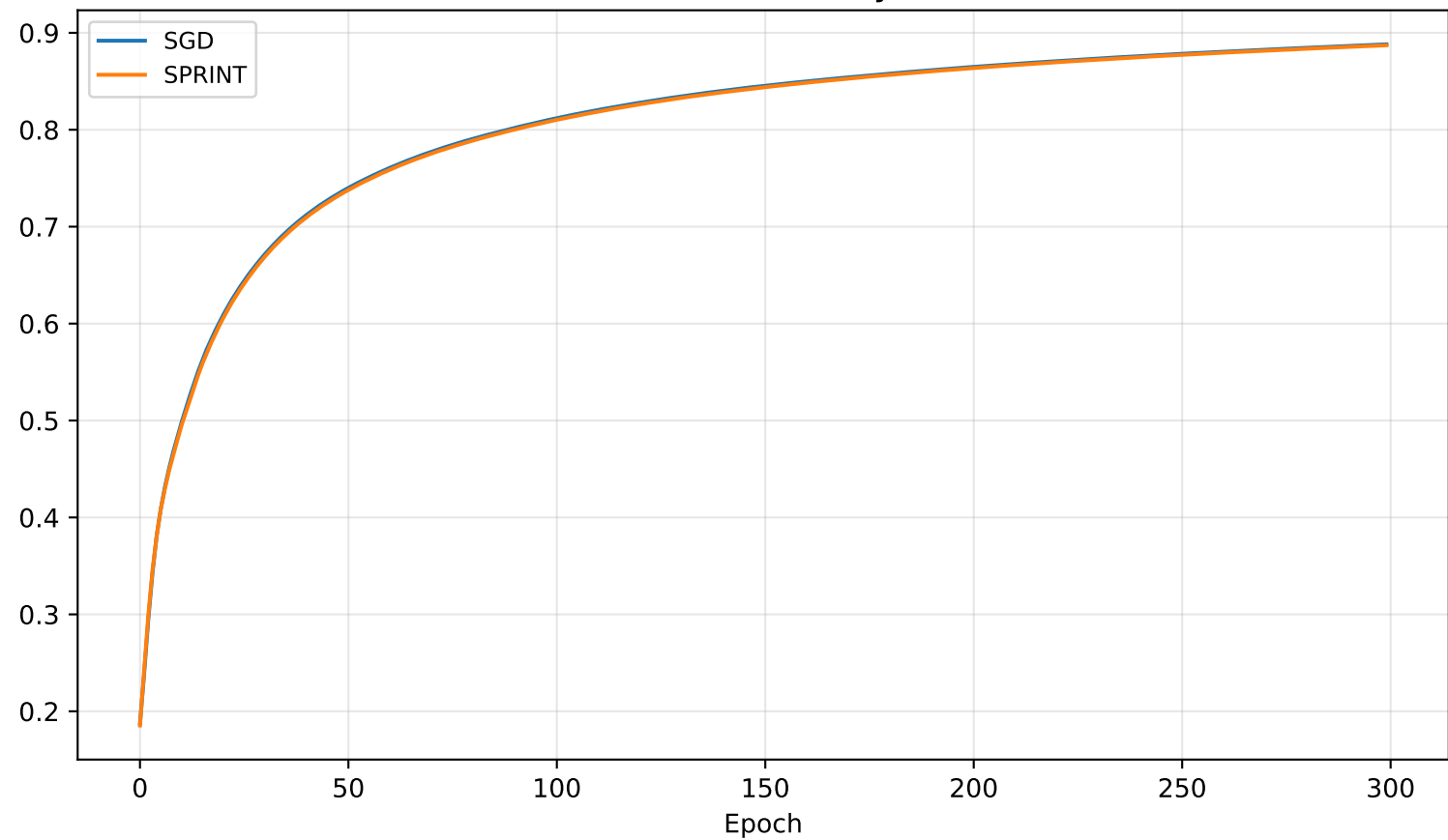
Train Accuracy
