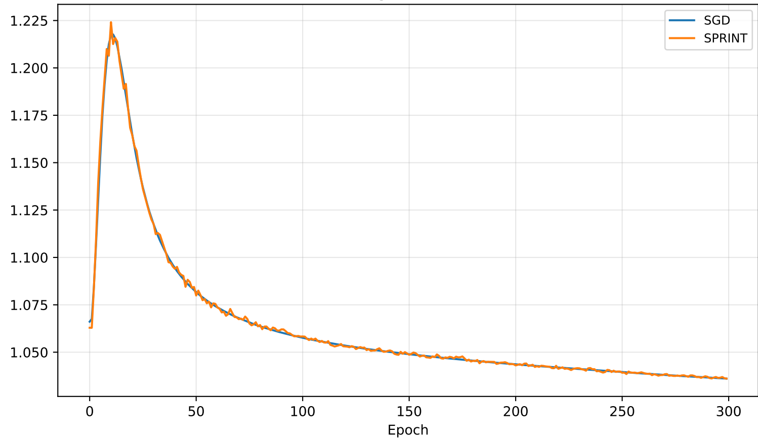
Weights Norm
