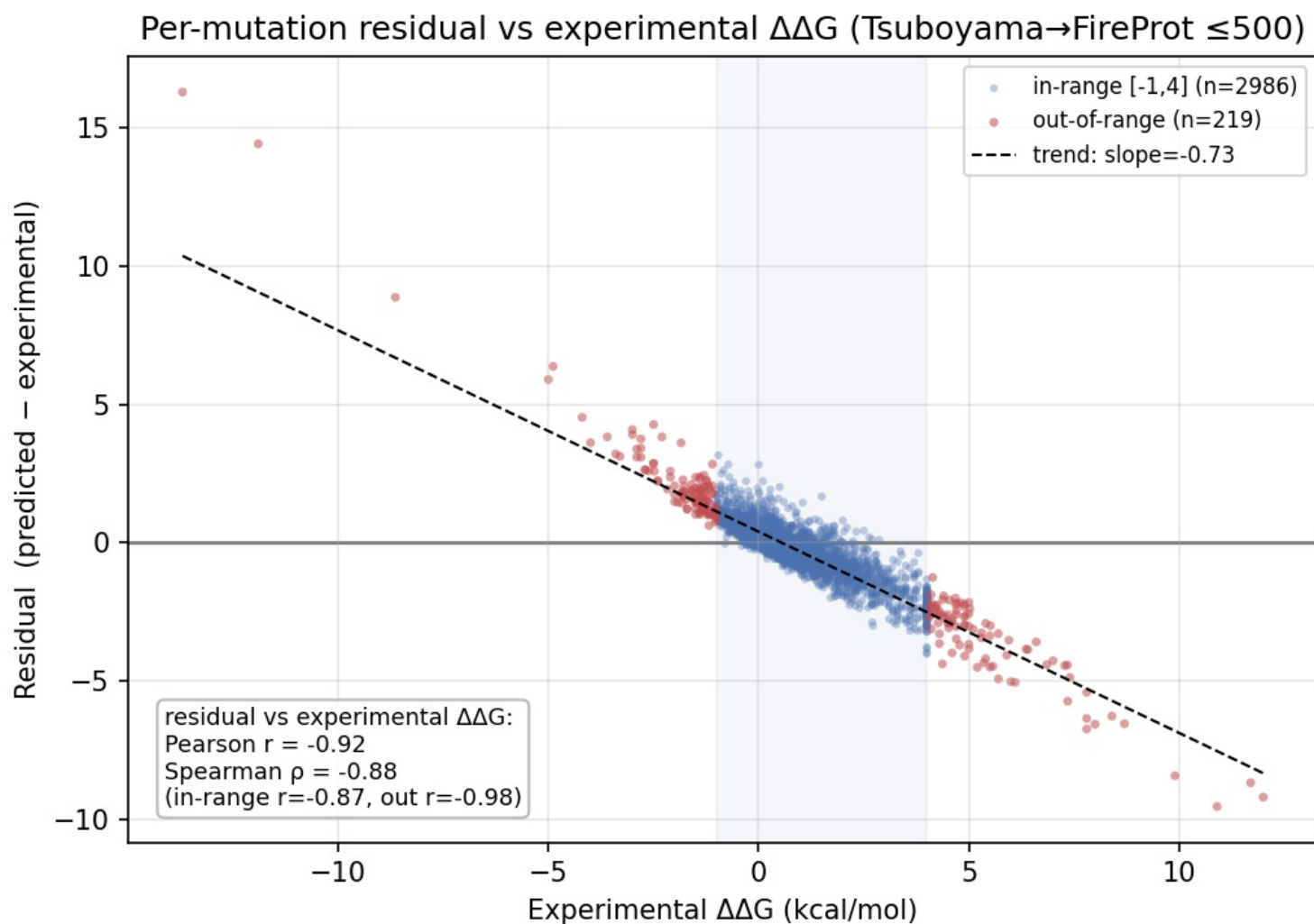
Figure 3. Per-mutation residual (predicted – experimental) vs experimental \Delta\Delta G . The residual is strongly anti-correlated with the true value ( Pearson r = -0.92 , Spearman \rho = -0.88 ; trend slope \approx -0.73 ): the model over-predicts strongly stabilizing mutations and under-predicts strongly destabilizing ones, crossing zero only near the dense training centre. In-range residuals cluster near zero (mean |residual| 0.69 kcal/mol, r = -0.87 ); out-of-range residuals fan out (mean |residual| 2.8, r = -0.98 ).
