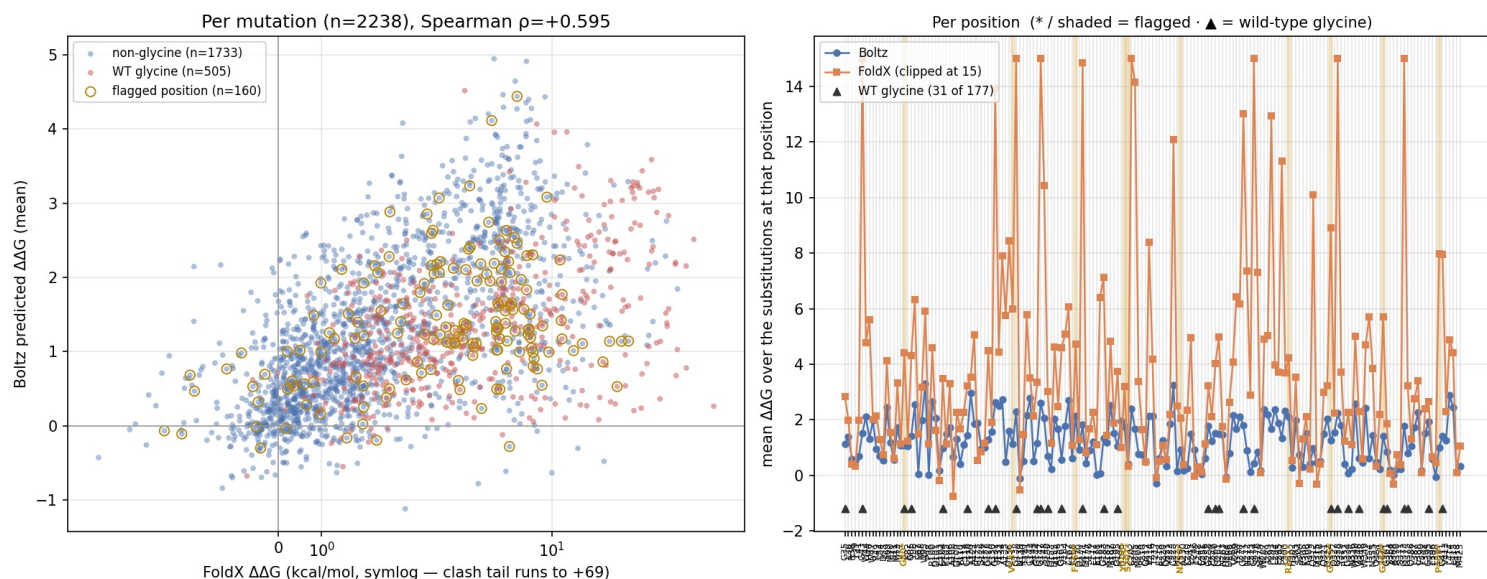
Figure 2. Left: per-substitution comparison; the horizontal axis is symlog because FoldX extends to tens of kcal/mol. Right: per-position means, with glycine sites marked. Agreement is visibly tighter away from glycine positions.
