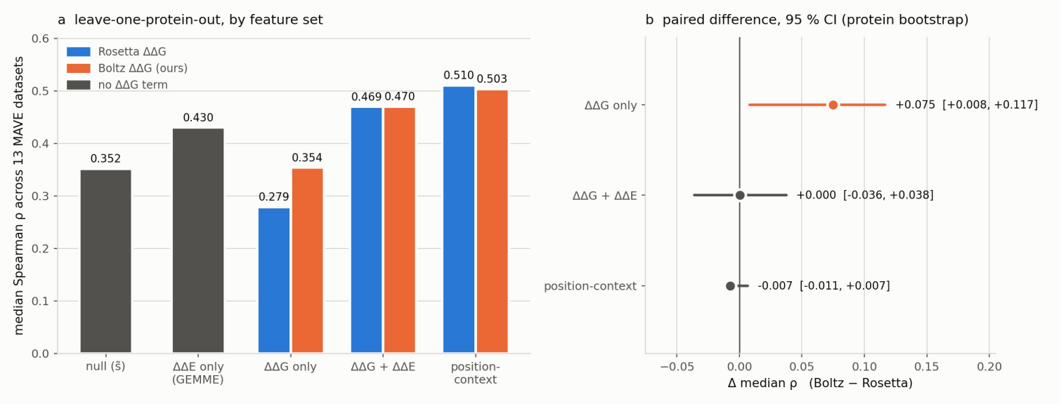
Figure 1. Leave-one-protein-out performance by feature set, both arms, and the paired difference with its 95 % protein-bootstrap interval. Grey bars carry no \Delta\Delta G term and are therefore arm-agnostic. Only \Delta\Delta G -only clears zero.
