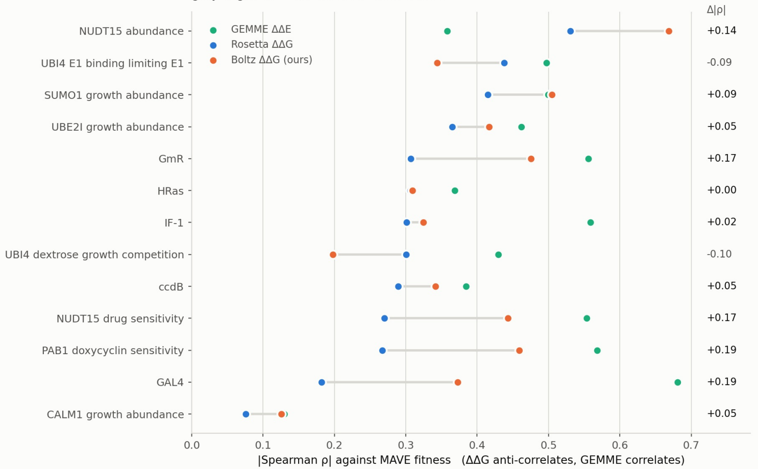
Figure 2. The same comparison with no model: direct |Spearman \rho | per dataset. Median |\rho| is 0.301 for Rosetta, 0.373 for ours and 0.497 for GEMME conservation.
