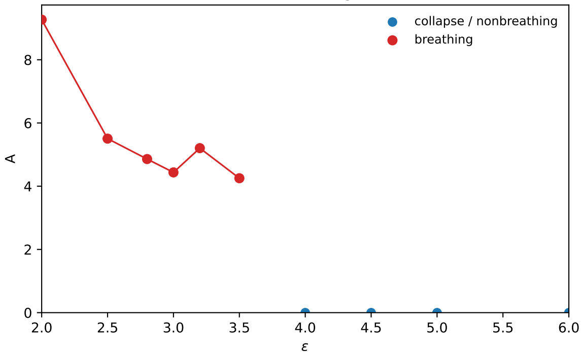
Bifurcation diagram
