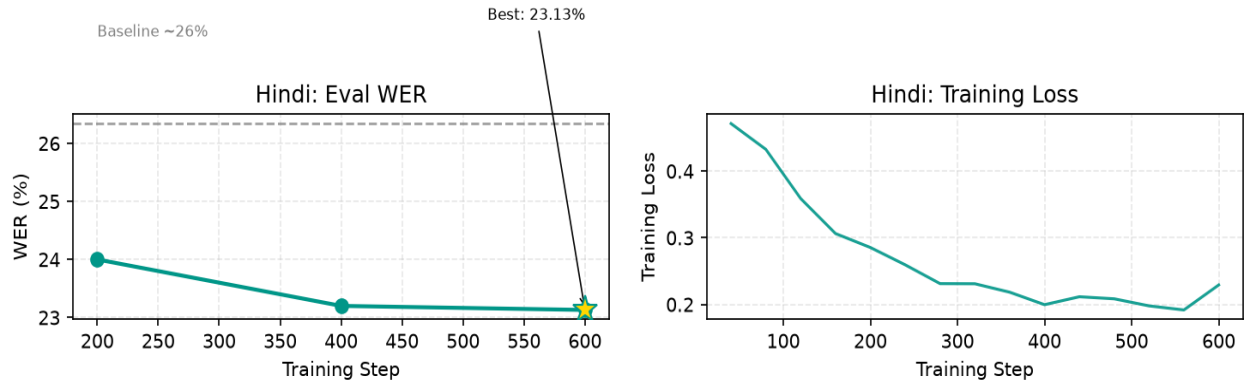
Figure: Hindi training curves. Left: eval WER (star = deployed checkpoint). Right: training loss per step.
