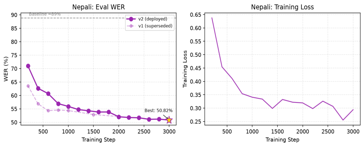
Figure: Nepali training curves. Left: eval WER (star = deployed checkpoint). Right: training loss per step.
