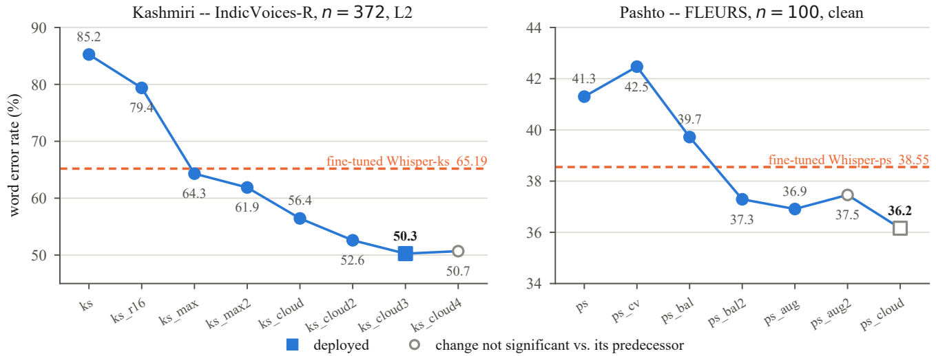
Figure 3: The two languages that took the most work, every run on one scorer. Kashmiri’s decisive moves are making the added language token trainable ( ks_max ) and repairing the subword vocabulary ( ks_cloud3 ); Pashto’s is noise-augmented training ( ps_aug ). Hollow markers are runs whose change from their predecessor does not survive a paired bootstrap—including the one we deployed.
