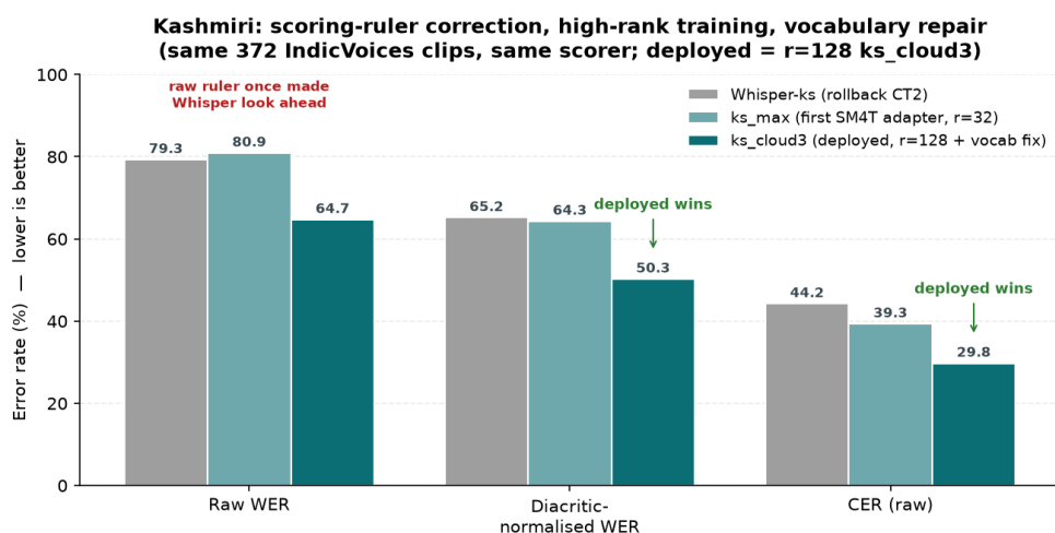
Figure 6: Same 372 IndicVoices clips, same scorer. Raw WER once made Whisper look ahead of the first adapter ( ks_max ) — an artefact of the Perso-Arabic scoring ruler. With the ruler corrected, every successive adapter widens the win; the deployed r=128 ks_cloud3 leads on all three measures.
