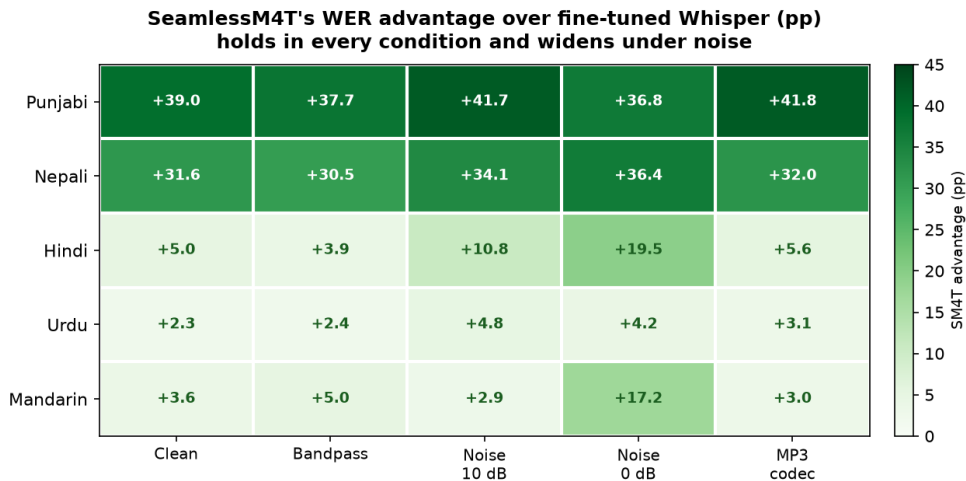
Figure 5: SeamlessM4T's WER advantage over fine-tuned Whisper (percentage points) across the five channel conditions. Positive everywhere; Hindi (+5.0→+19.5) and Mandarin (+3.6→+17.2) widen most at 0 dB SNR. This is the conservative zero-shot comparison — the deployed hi/ne LoRA adapters improve on it further.
