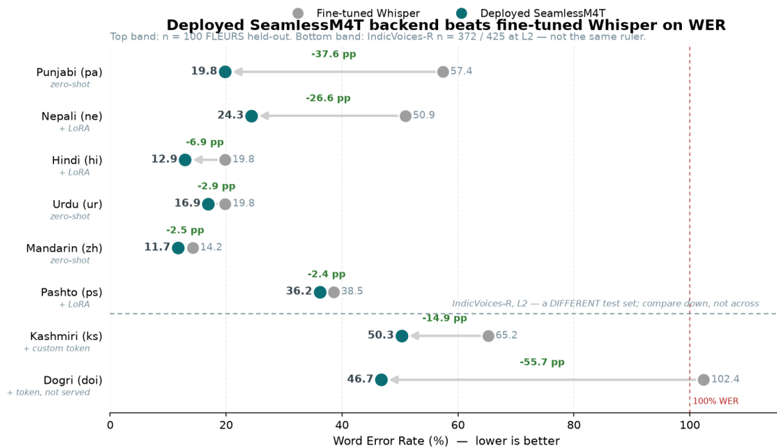
Figure 4: Deployed SeamlessM4T backend vs the fine-tuned Whisper model, for all eight languages. Every arrow points to the deployed backend — lower WER in every case. The two bands are different test sets and must not be compared across. The top six are FLEURS held-out, n=100. Kashmiri and Kashmiri's neighbour Dogri are absent from FLEURS entirely, so the bottom two are the IndicVoices-R test splits (n=372 and n=425) scored at L2 — read them down their own column. Dogri's 102.39% is what the deployed system actually did before it had a Dogri model: Whisper's language identification misrouted the audio and produced more errors than there were reference words, which is why that bar crosses the 100% line. Dogri's 46.73% is its best model, which is trained but NOT yet served ($4.5).
