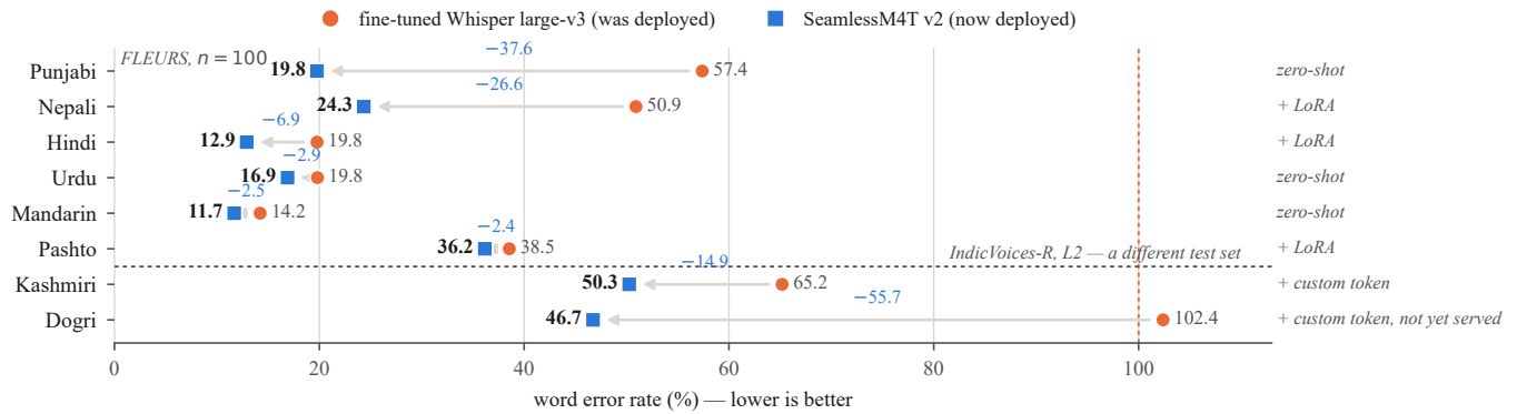
Figure 1: Backend replacement across all eight languages. Every language moves left, and three of the six FLEURS languages needed no adaptation at all—zero-shot SeamlessM4T already beat a Whisper model fine-tuned on that language. The lower band is a different test set: Kashmiri and Dogri are absent from FLEURS and are scored on IndicVoices-R at L2, so those two rows are comparable down the column but not across to the six above. Dogri’s “before” is what the deployed system actually did—misroute the audio to Whisper’s language identification—which is why it starts beyond 100%.
