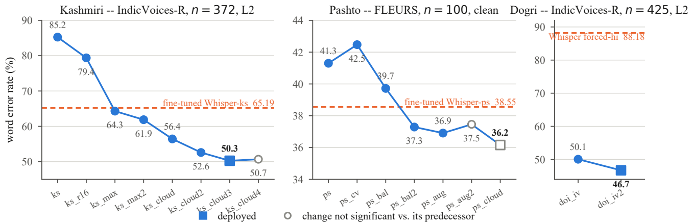
Figure 3: Every adaptation run for the three languages that needed more than one, each panel on its own single scorer. Kashmiri’s decisive moves are making the added language token trainable (ks_max) and repairing the subword vocabulary (ks_cloud3); Pashto’s is noise-augmented training (ps_aug); Dogri’s two runs differ only in being allowed to finish, and replicate Kashmiri’s convergence result on a different script and corpus. Hollow markers are runs whose change from their predecessor does not survive a paired bootstrap—including the one we deployed.
