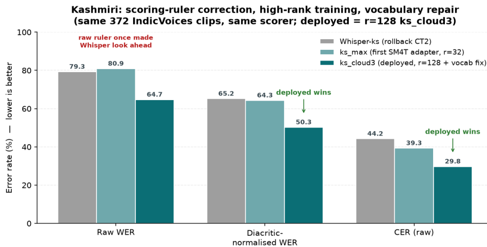
Figure 6: Same 372 IndicVoices clips, same scorer. Raw WER once made Whisper look ahead of the first adapter (ks_max) — an artefact of the Perso-Arabic scoring ruler. With the ruler corrected, every successive adapter widens the win; the deployed r=128 ks_cloud3 leads on all three measures.
