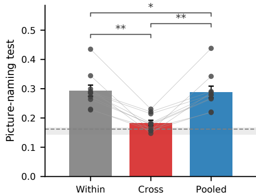
Category-independent balanced accuracy
