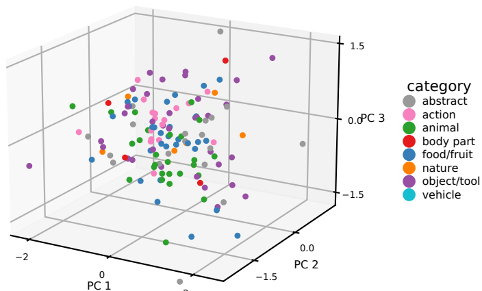
Auditory decoder (n=51)
