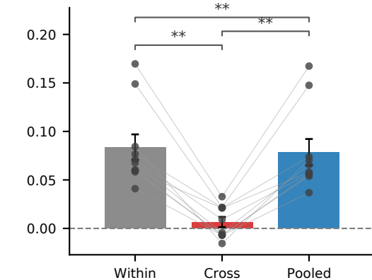
Cosine similarity
