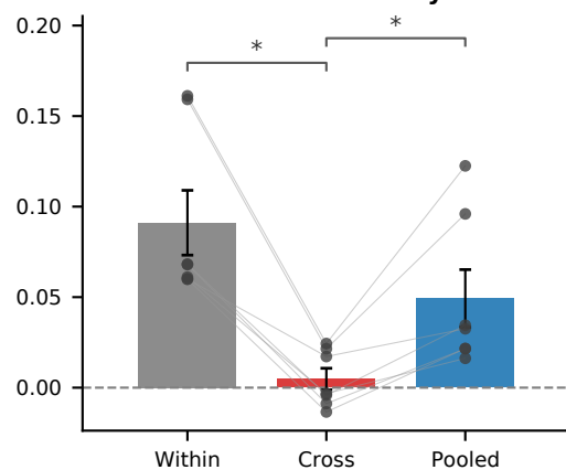
Cosine similarity
