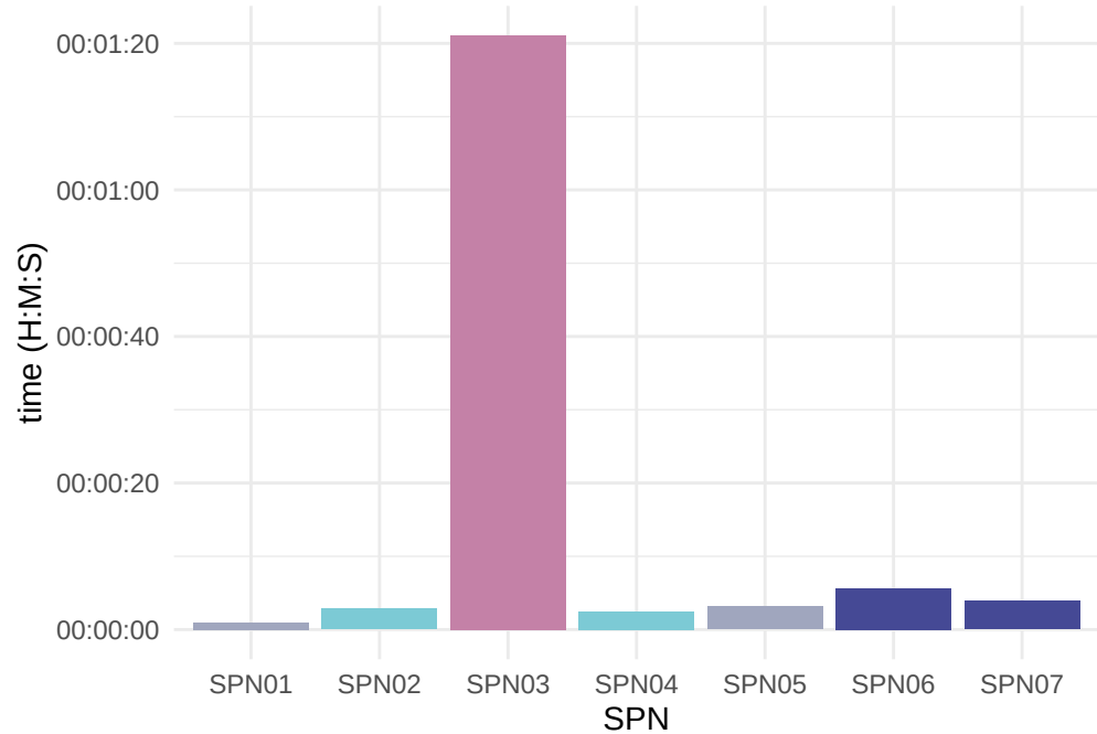
Simulate tissue
