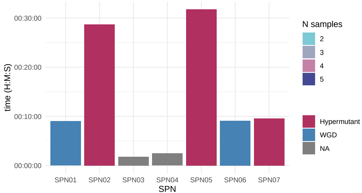
Simulate Mutations
