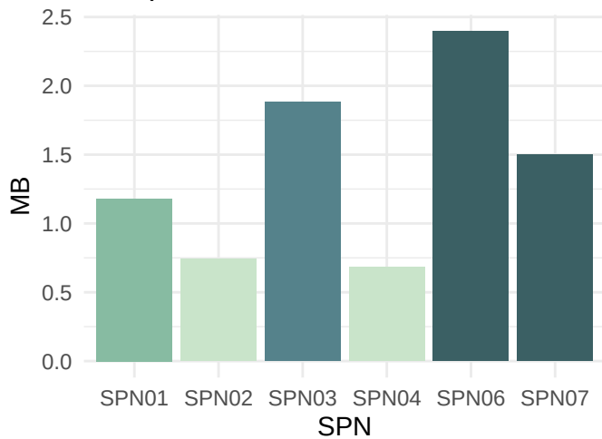
Sample Forest
