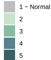
N samples
