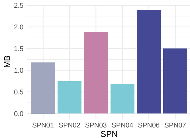
Sample Forest
