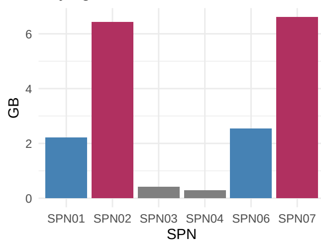
Phylogenetic Forest
