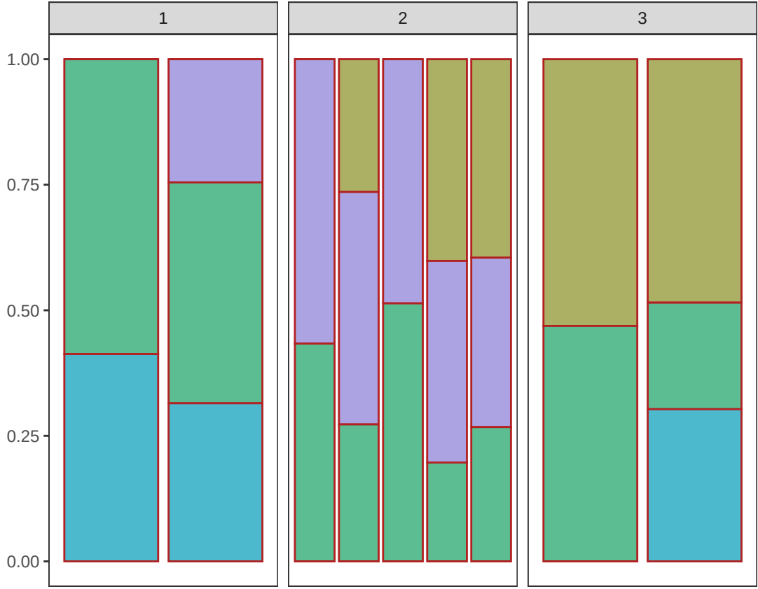
K-means clustering
