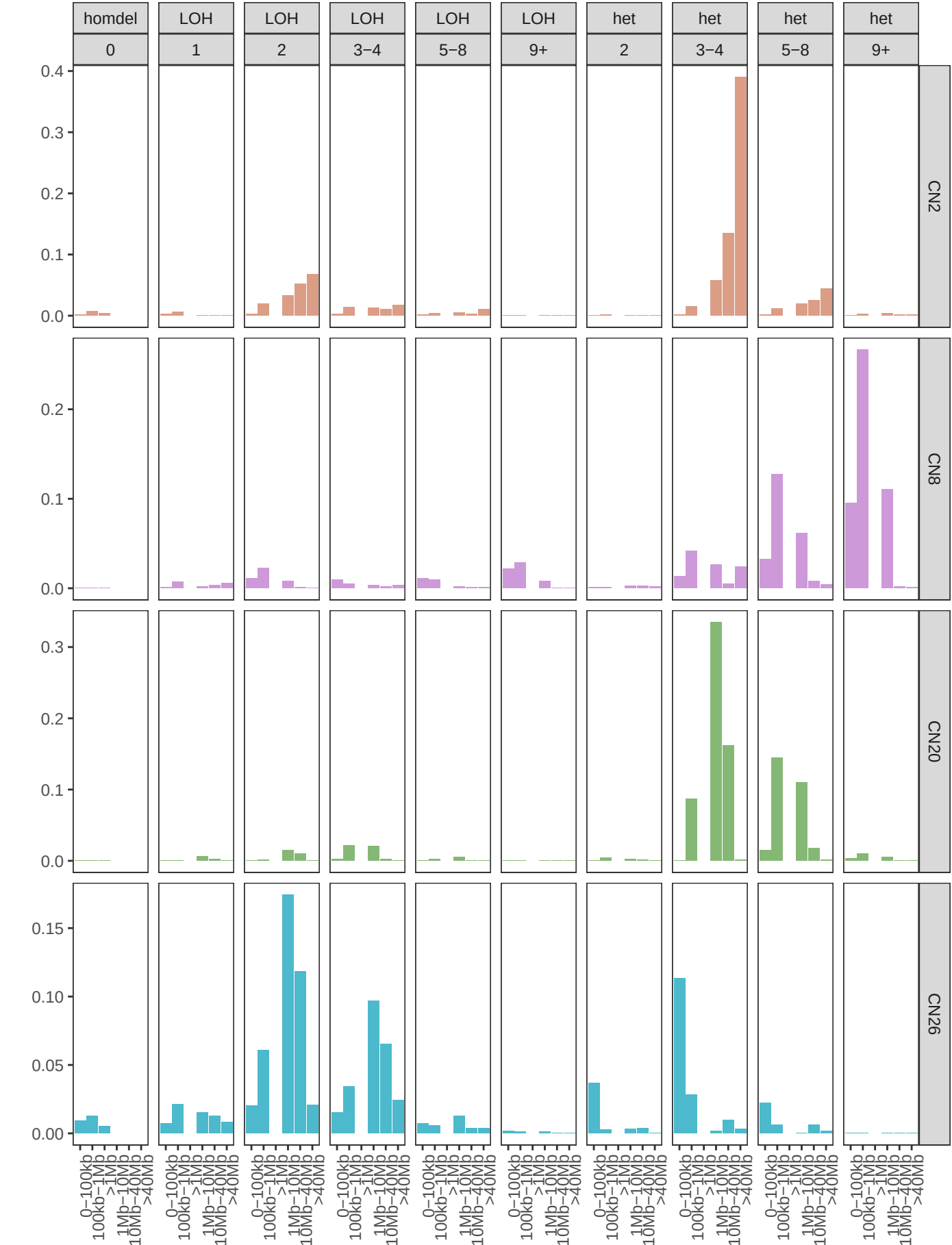
K-means clustering
