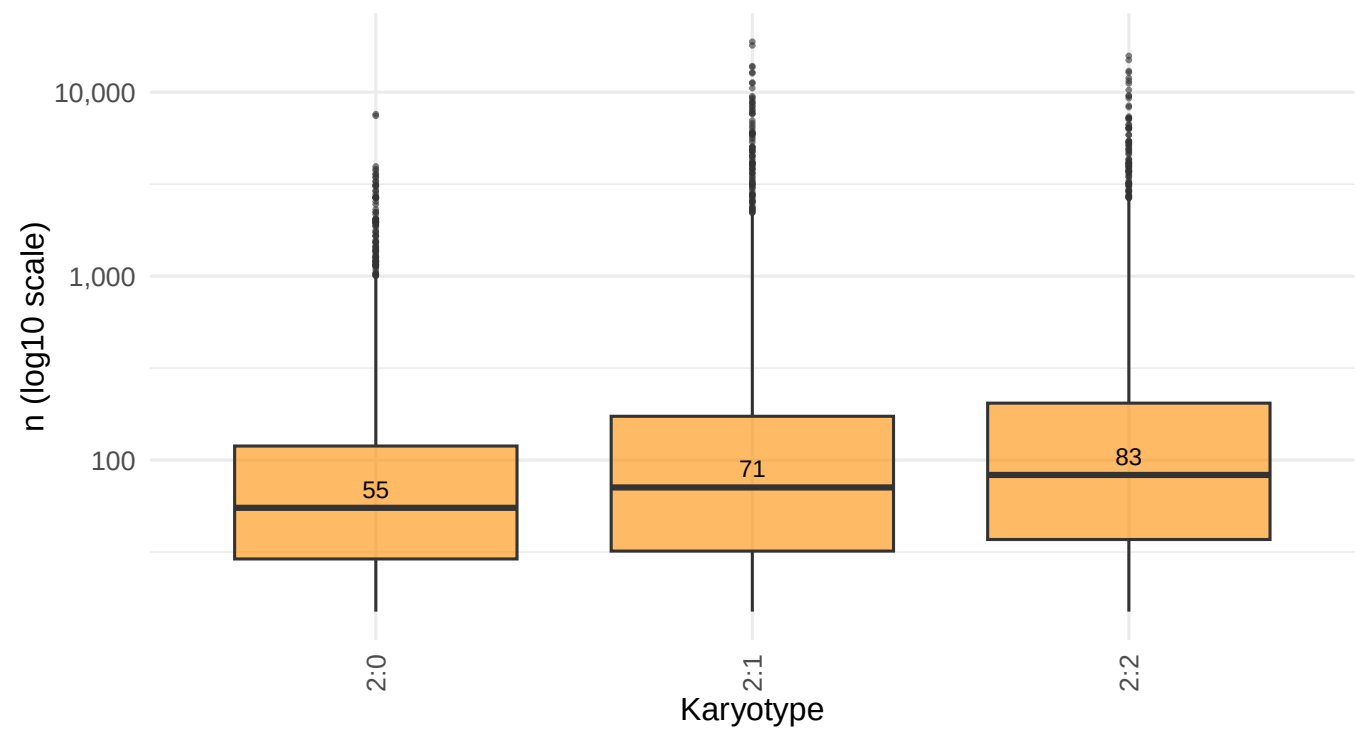
n distribution per karyotype (all samples)
