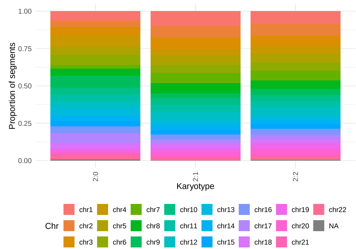
Chromosome composition per karyotype (proportion, all samples)
