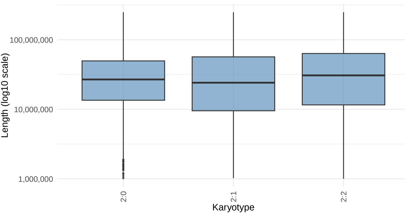
Segment length distribution per karyotype (all samples)
