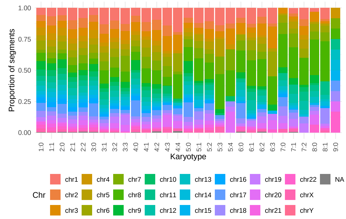
Chromosome composition per karyotype (proportion, all samples)
