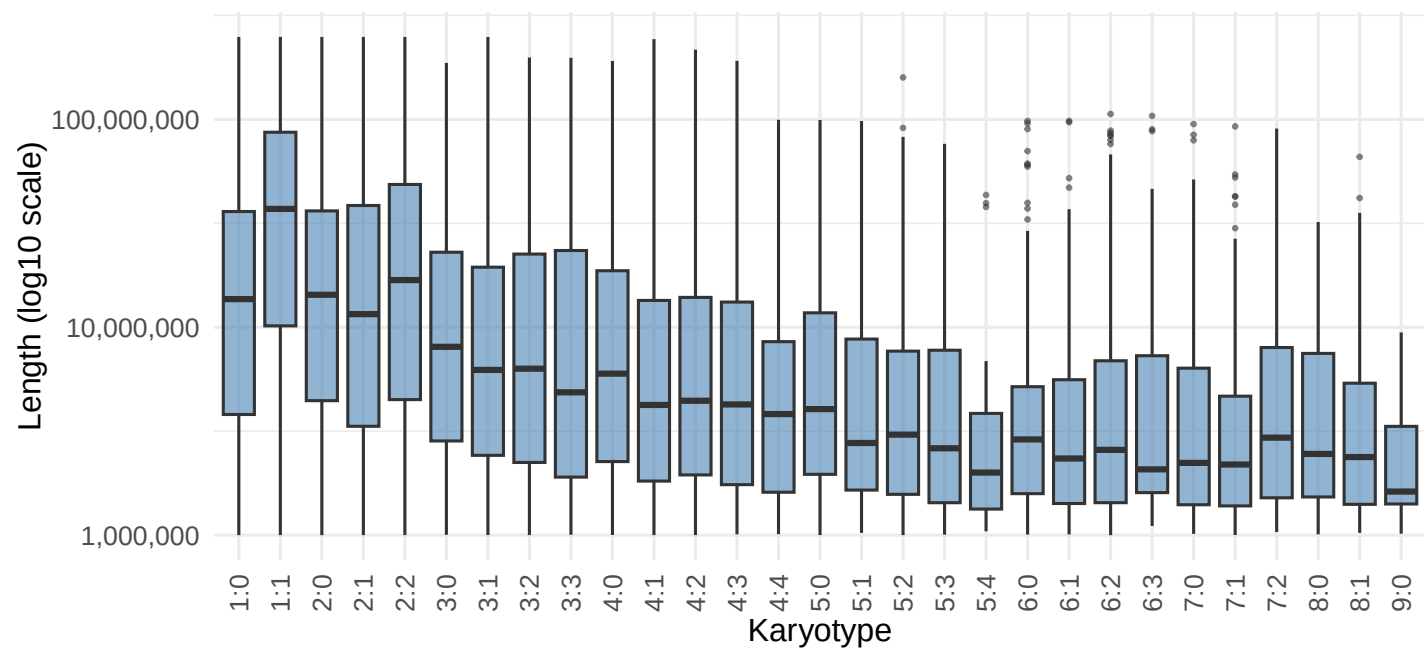
Segment length distribution per karyotype (all samples)
