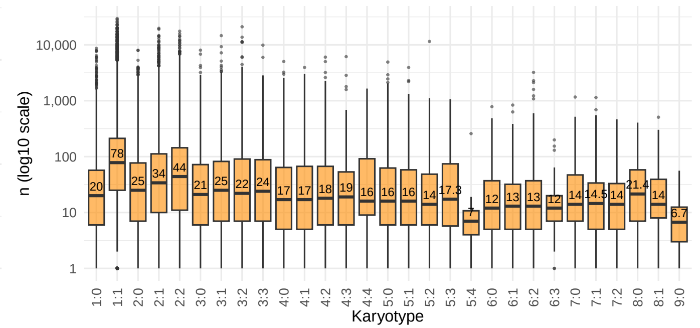
n distribution per karyotype (all samples)
