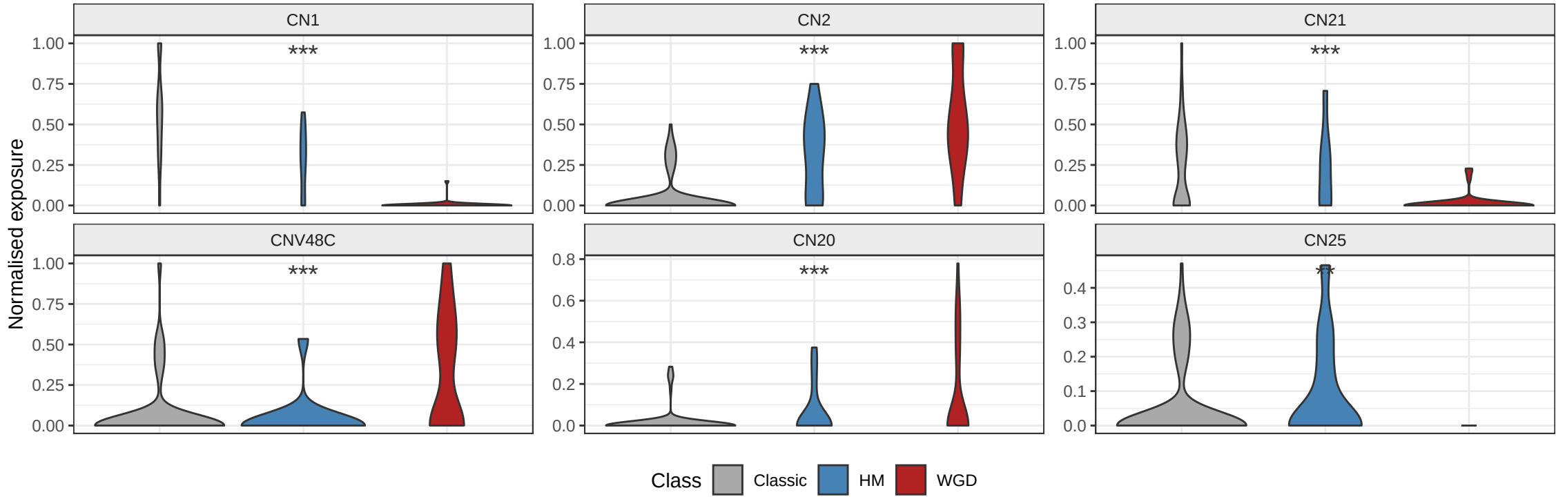
CN signature exposure by class KW adjusted p-value: *** <0.001, ** <0.01, * <0.05, ns
